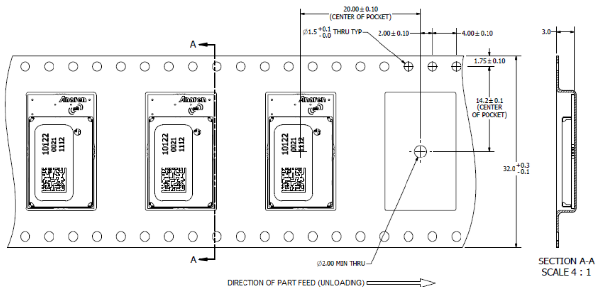
Figure 11 A2541E24A00GR and A2541E24C00GR Tape-Reel Packaging Detail (500/Reel)
