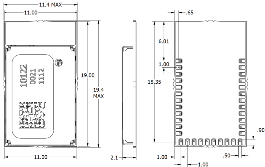
Figure 8 A2541E24A dimensions
