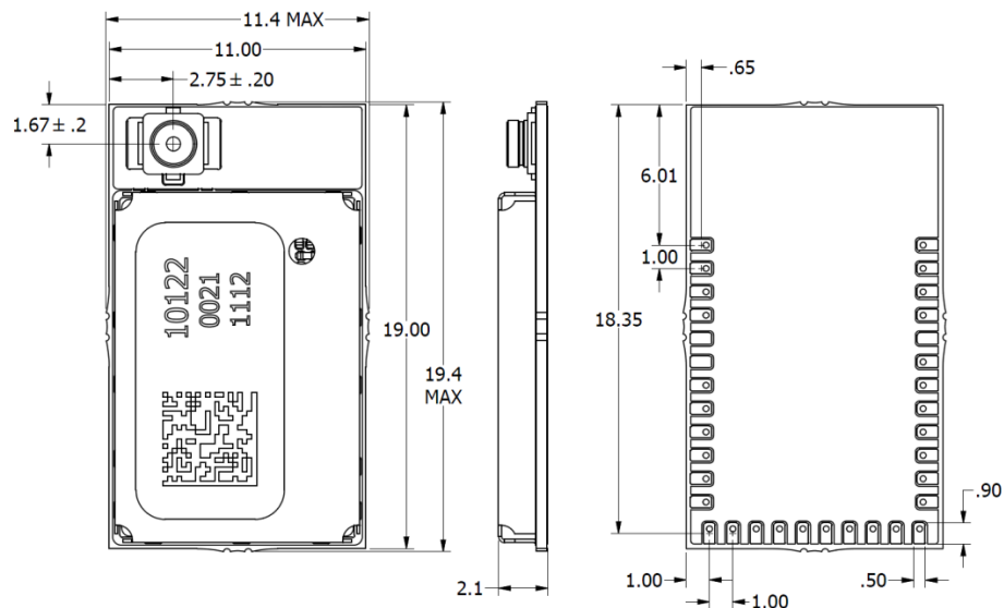
Figure 9 A2541E24C dimensions
