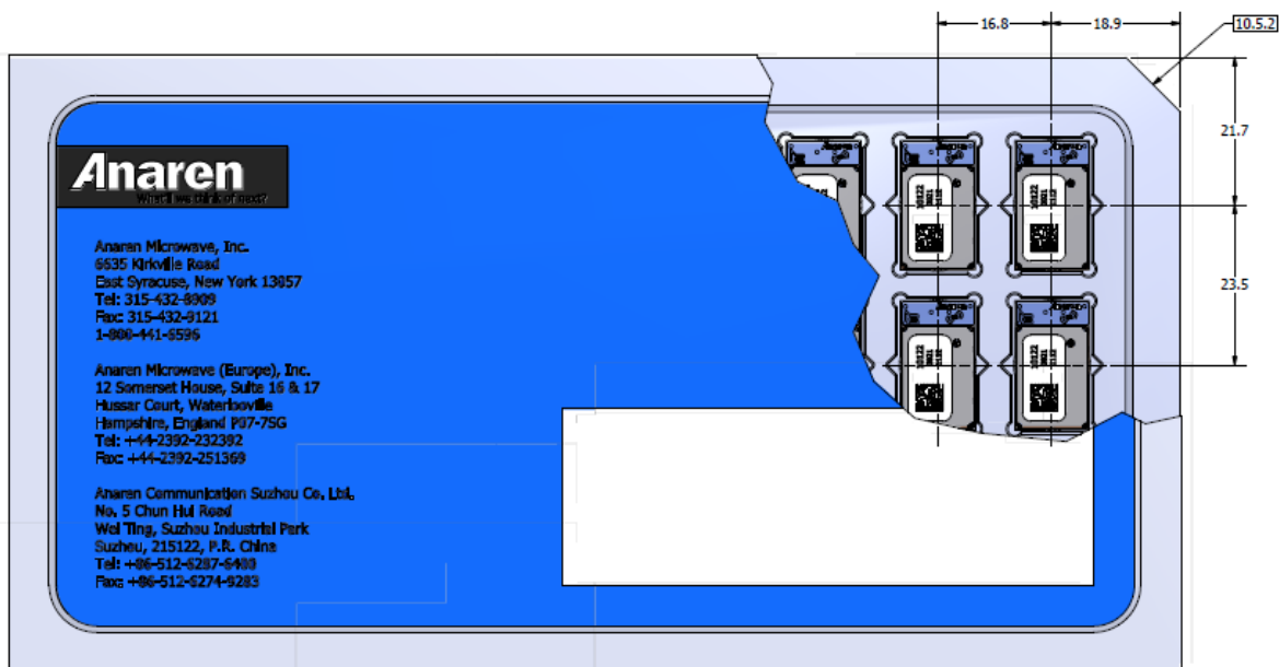
Figure 10 A2541E24A00GM and A2541E24C00GM Matrix Tray Packaging Detail (27/Tray)
