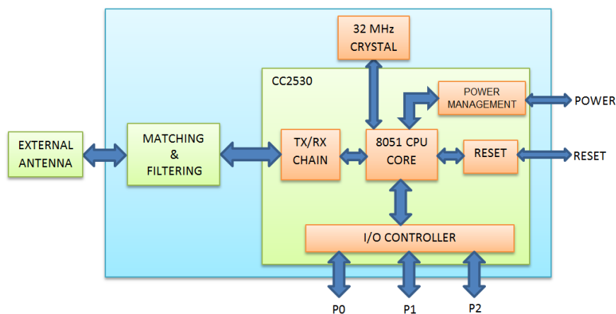
Figure 2 The functionality of the A2530R24C, using an external antenna
