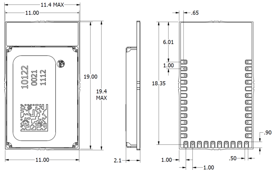
Figure 8 A2530R24A dimensions
