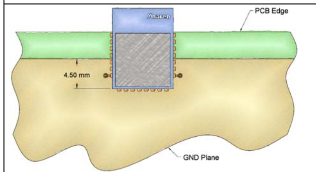
Figure 9 Mounting the module along an edge with overhang. This option is not generally recommended, but is a method to save PCB in an environmentally benign environment
