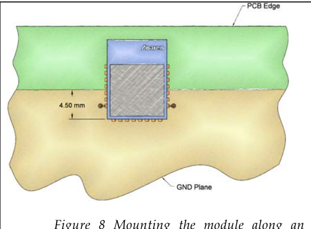
Figure 8 Mounting the module along an edge
