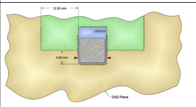
Figure 10 Mounting the module along an edge, with a ground plane cut-out. This option degrades range slightly.
