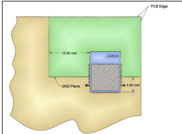
Figure 7 Mounting the module in a corner
