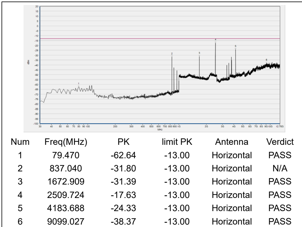
(GPRS 850MHz, Channel = 190, Horizontal)
