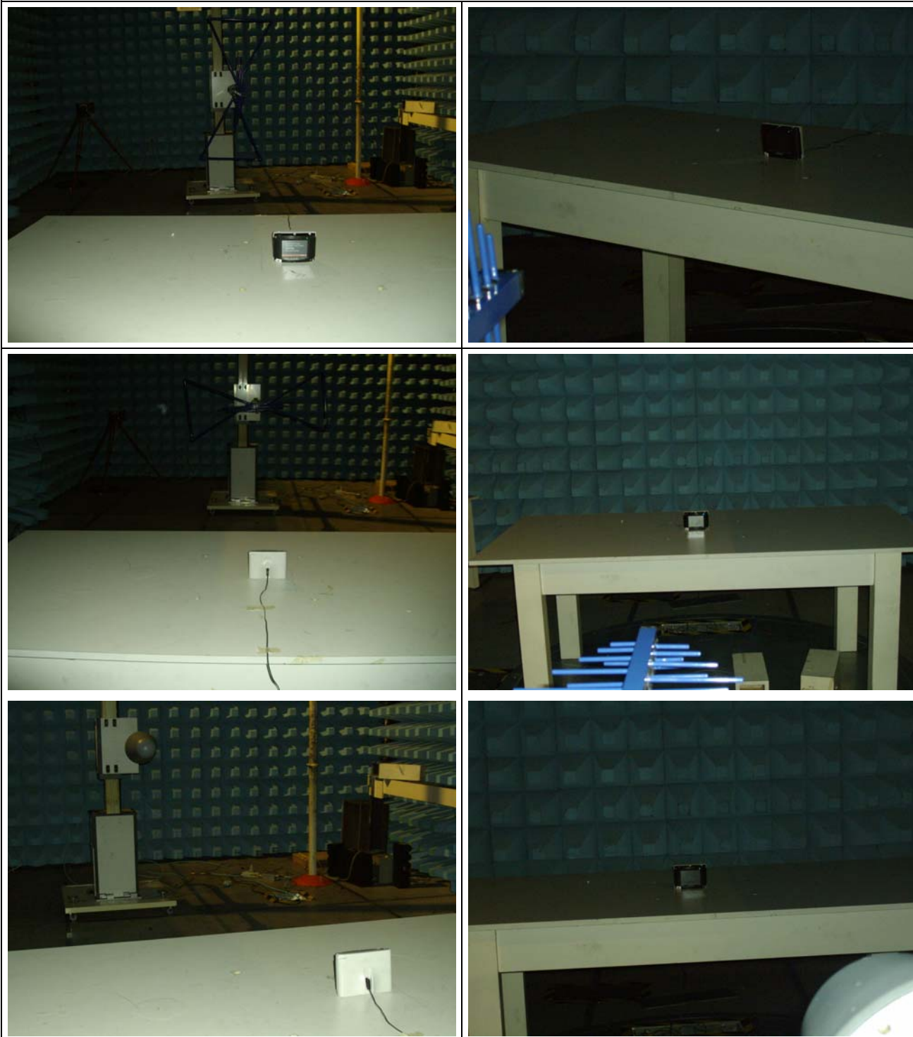
PHOTO 3 – SET-UP FOR EMISSION RADIATED TEST
