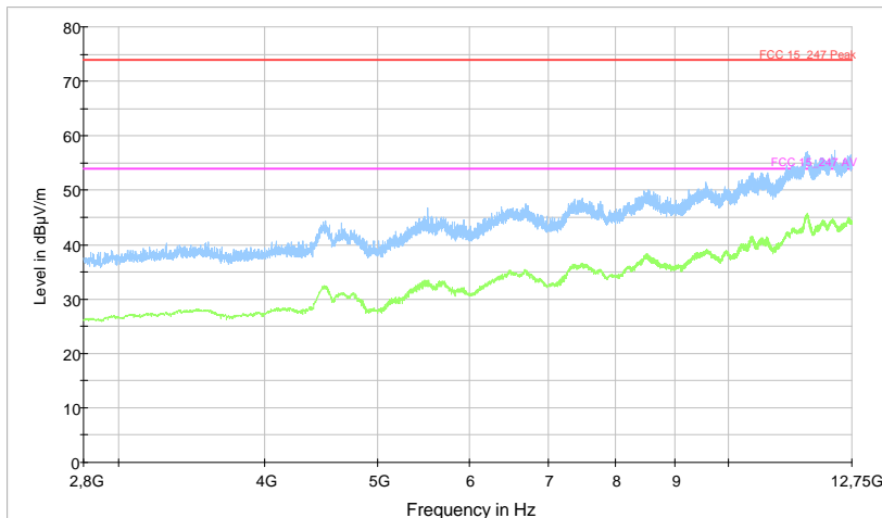
FCC_15_247_RADIATED_SPURIOUS_VERTICAL
