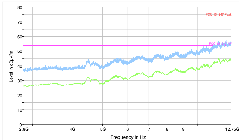
FCC_15_247_RADIATED_SPURIOUS_VERTICAL
