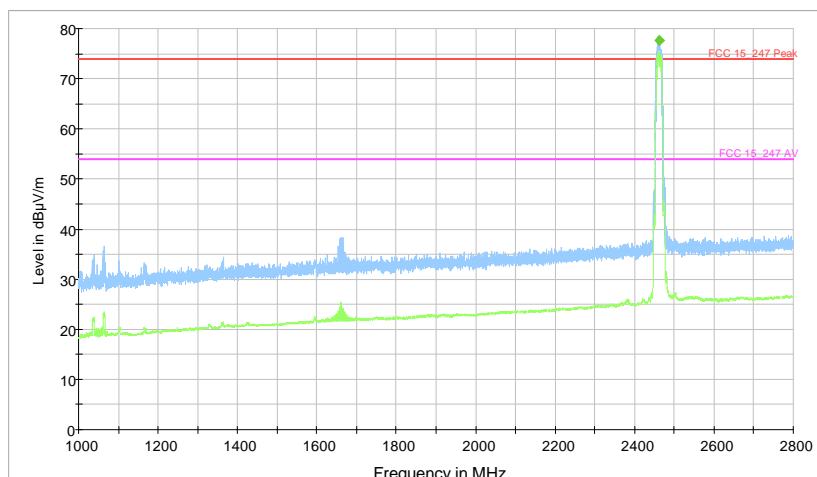
FCC_15_247_RADIATED_SPURIOUS_HORIZONTAL
