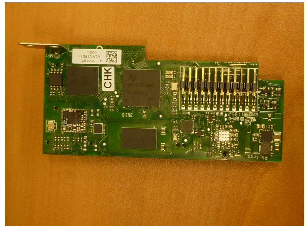
EPCOS – front detail – metal shield removed
