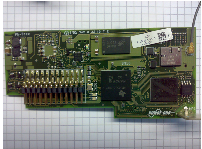
EPCOS – FRONT DETAIL
