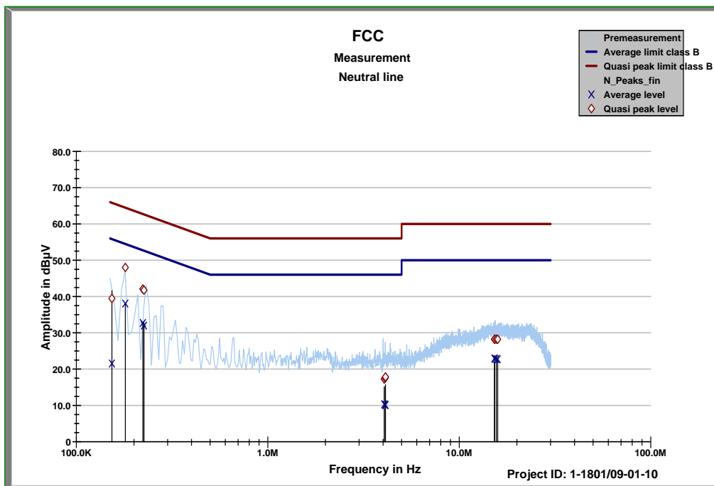
Plot 2: TX CH00, neutral line
