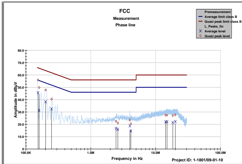
Plot 3: Idle, phase line
