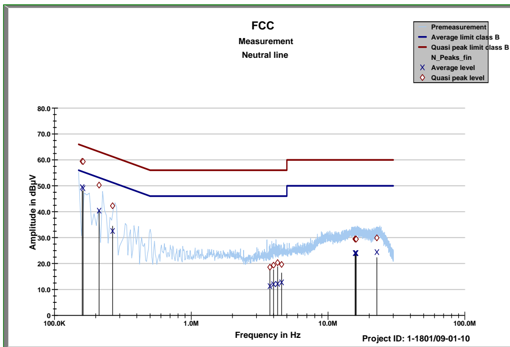
Plot 4: Idle, neutral line
