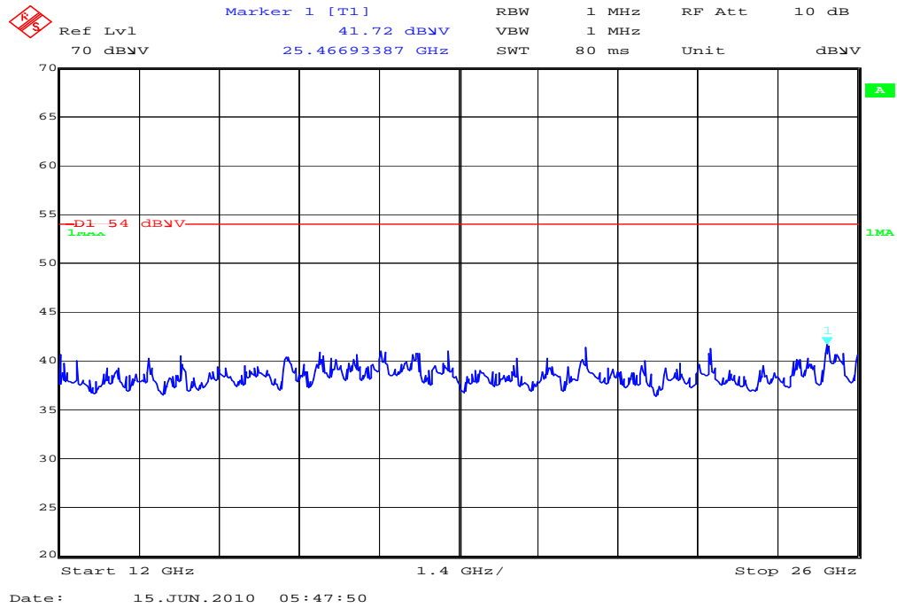
Plot 5: Idle, 12 – 26GHz, vertical/horizontal max.hold
