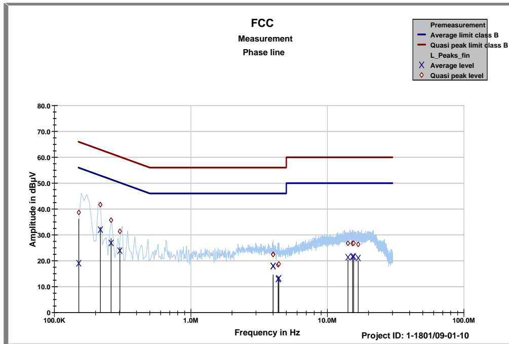
Plot 1: TX CH00, phase line
