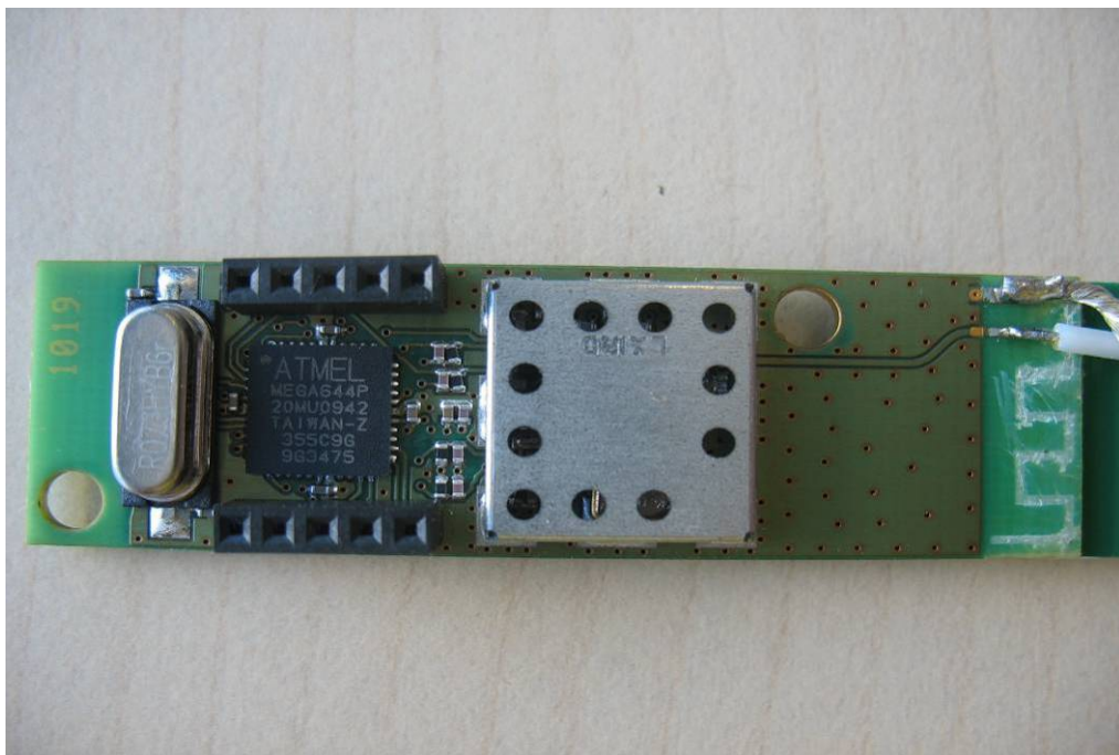
Photo 10: Conducted sample
