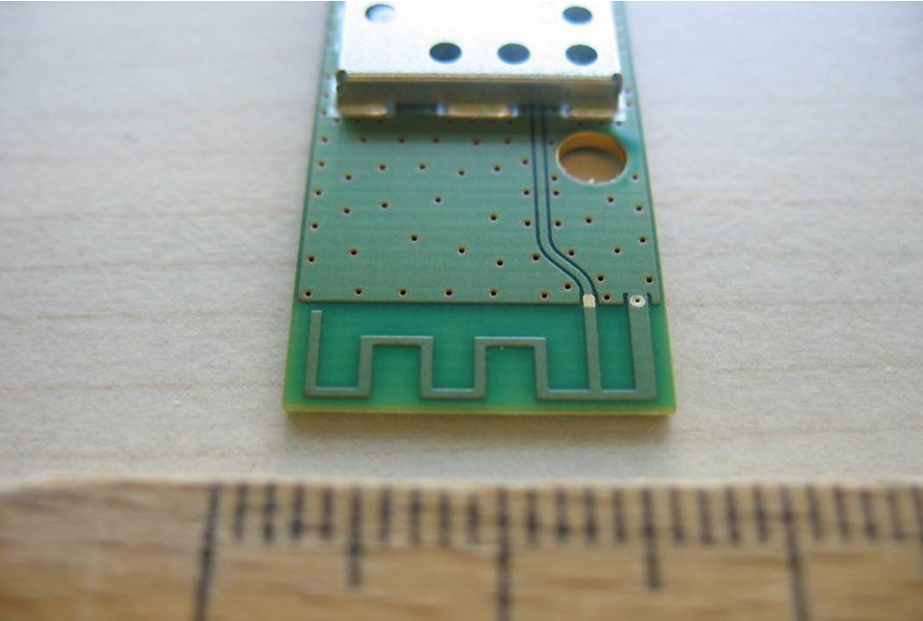
Photo 3: Radiated sample
