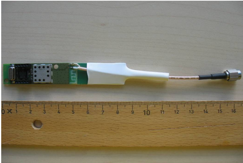
Photo 9: Conducted sample
