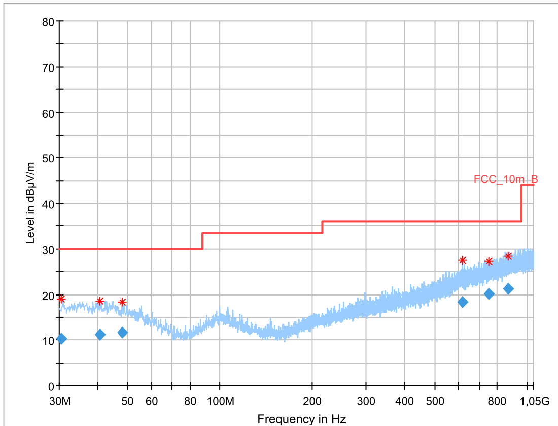
Plot 1: 30 MHz to 1 GHz, TX mode, 2402 MHz, vertical & horizontal polarization
