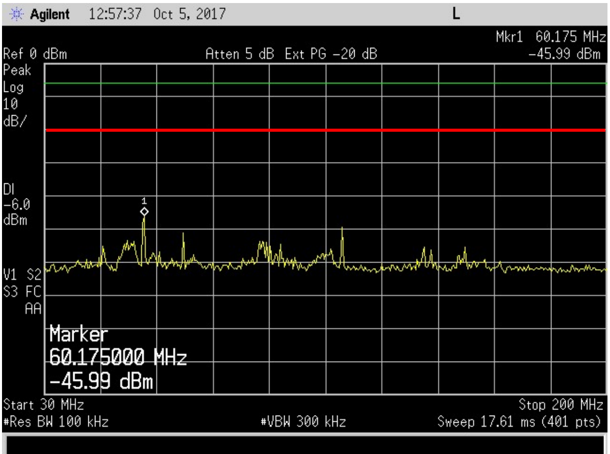
Figure 5. Antenna Conducted Emissions Mid Channel, 30 – 200 MHz
