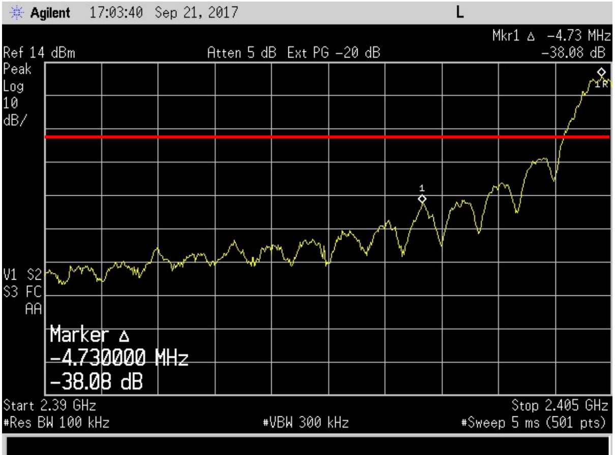
Figure 11. Band Edge Compliance, Low Channel Delta - Peak
