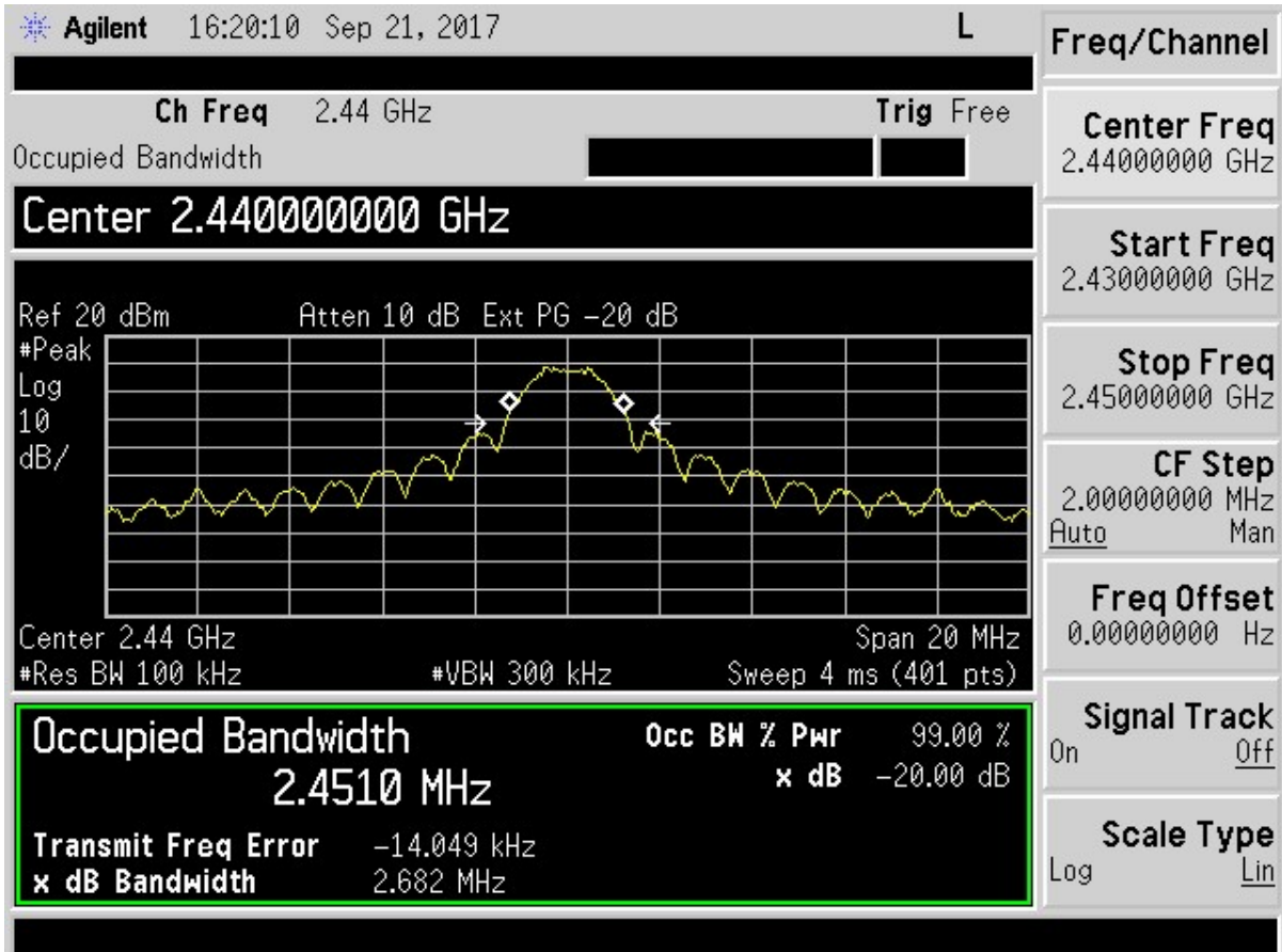
Figure 21.20 dB Bandwidth – Mid Channel
