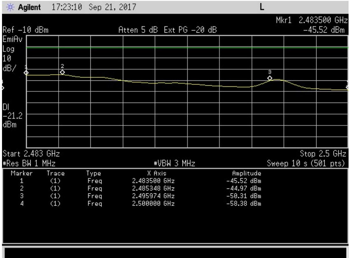
Figure 16. Conducted Restricted Measurements AVG, 2.4835 GHz to 2.5 GHz
