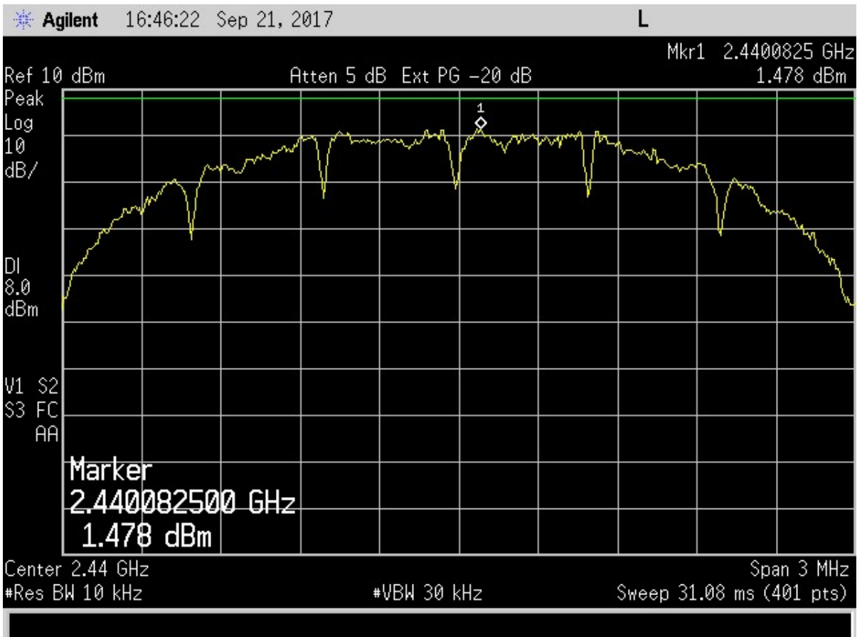
Figure 27. Power Spectral Density - Part 15.247 (e) - Mid Channel
