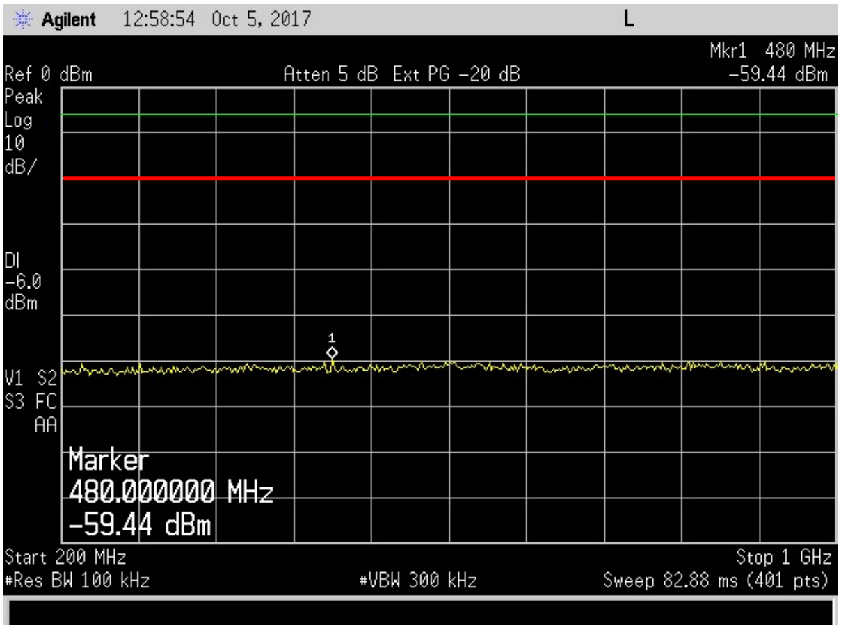
Figure 6. Antenna Conducted Emissions Mid Channel, 200 – 1000 MHz
