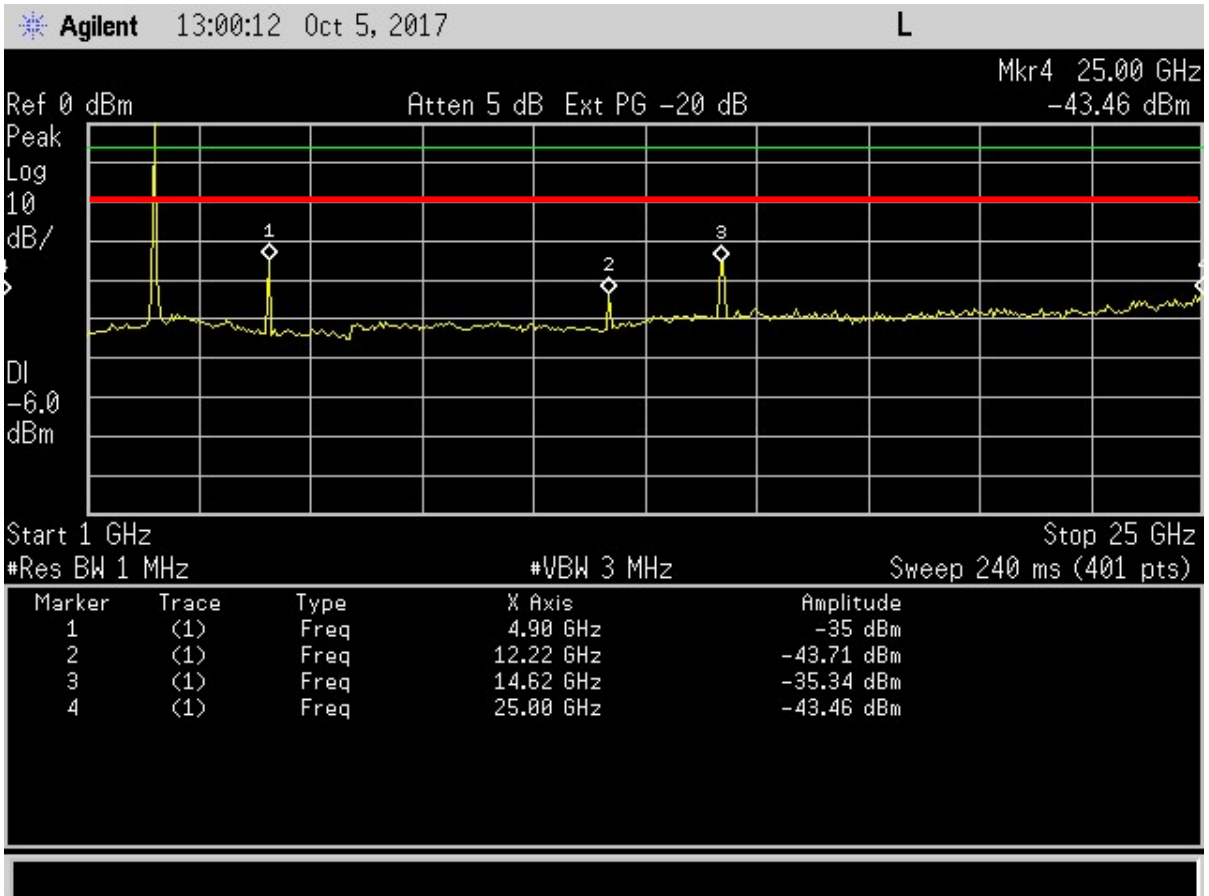
Figure 7. Antenna Conducted Emissions Mid Channel, 1 GHz – 25 GHz
