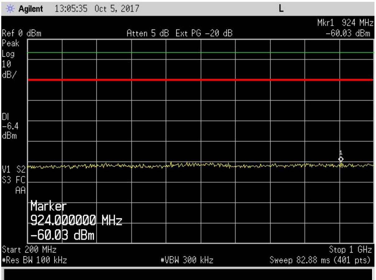
Figure 9. Antenna Conducted Emissions High Channel, 200 – 1000 MHz
