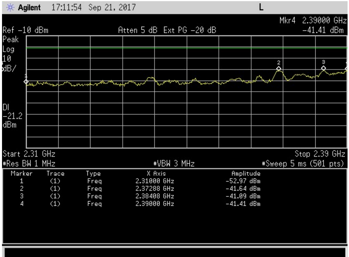
Figure 12. Conducted Restricted Band Measurements 2.31 GHz to 2.39 GHz
