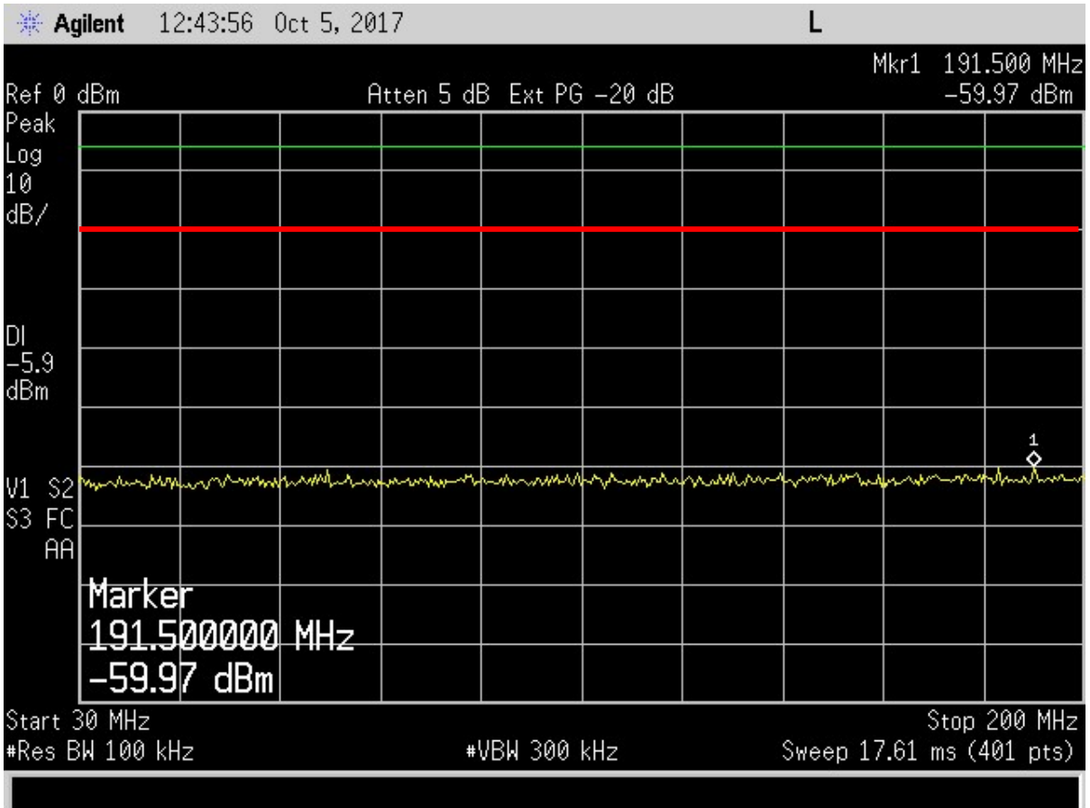
Figure 2. Antenna Conducted Emissions Low Channel, 30 – 200 MHz
