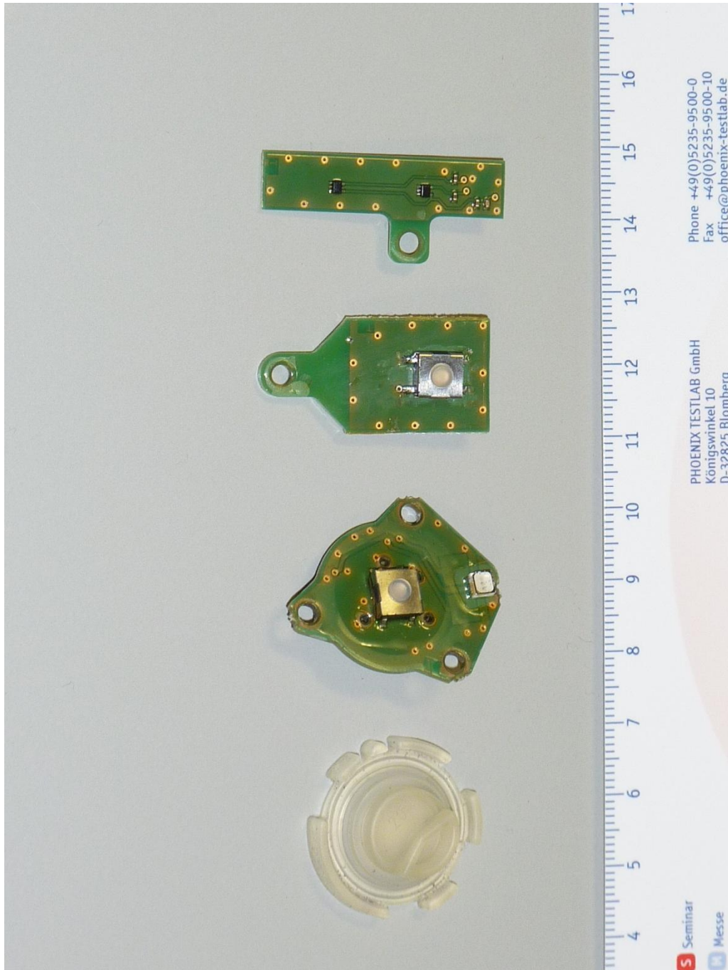
151497_n_11.JPG: FPS COM 7000, additional PCBs, bottom view
