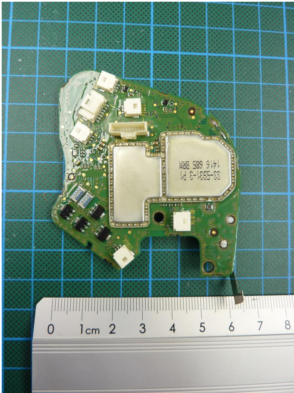
151497_n_2.JPG: FPS COM 7000, PCB1, bottom view
