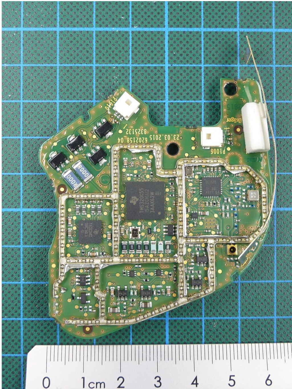
151497_n_6.JPG: FPS COM 7000, PCB1, top view, shielding removed
