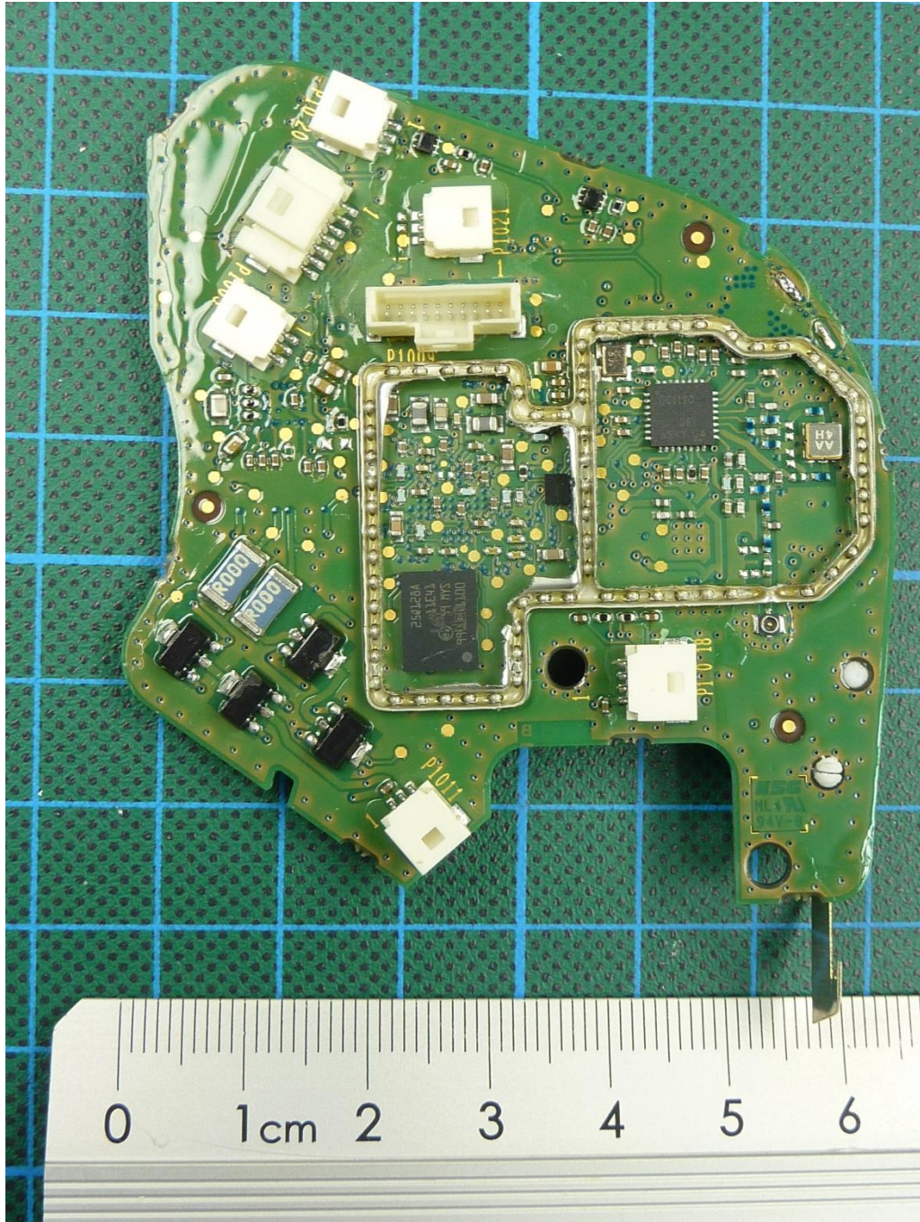
151497_n_5.JPG: FPS COM 7000, PCB1, bottom view, shielding removed
