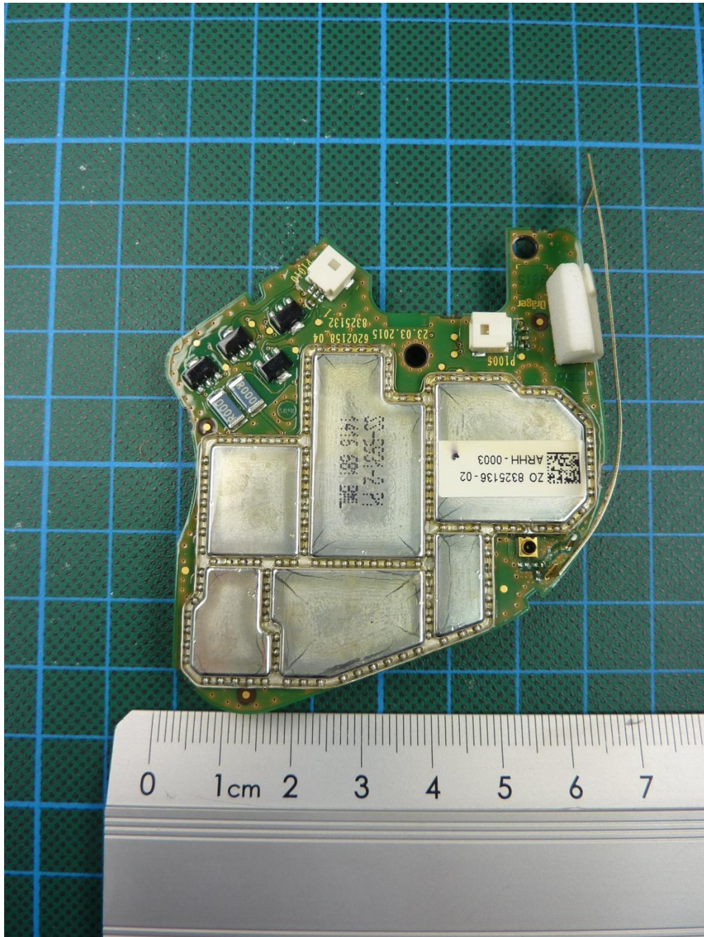
151497_n_1.JPG: FPS COM 7000, PCB1, top view
