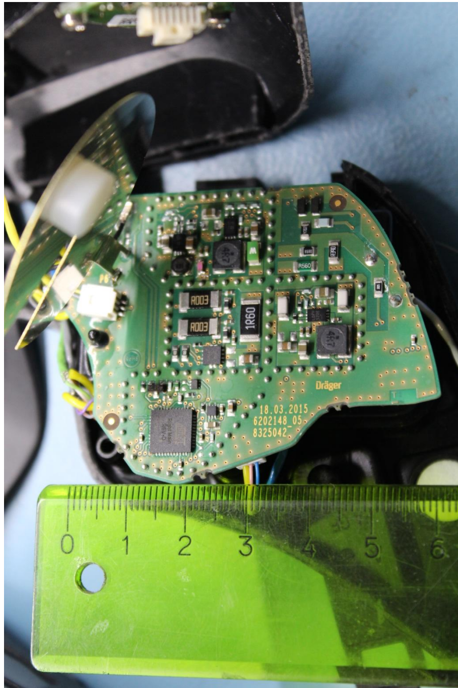
151497_n_12.JPG: FPS COM 7000, PCB2, top view, unspotted sample (supplied by the applicant)
