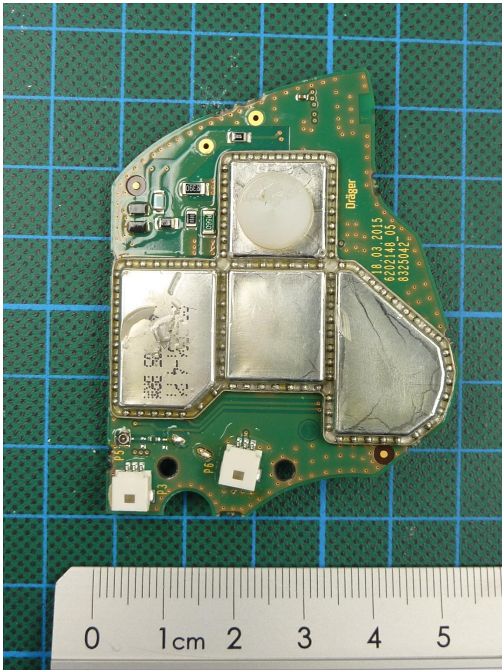
151497_n_8.JPG: FPS COM 7000, PCB2, top view, antenna removed
