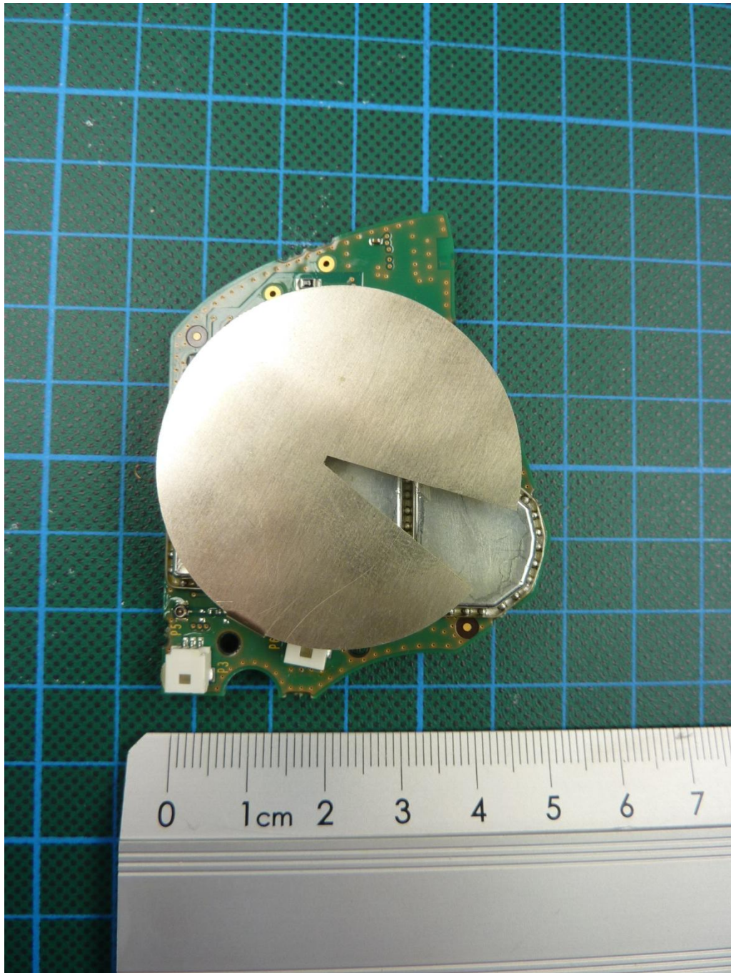
151497_n_3.JPG: FPS COM 7000, PCB2, top view
