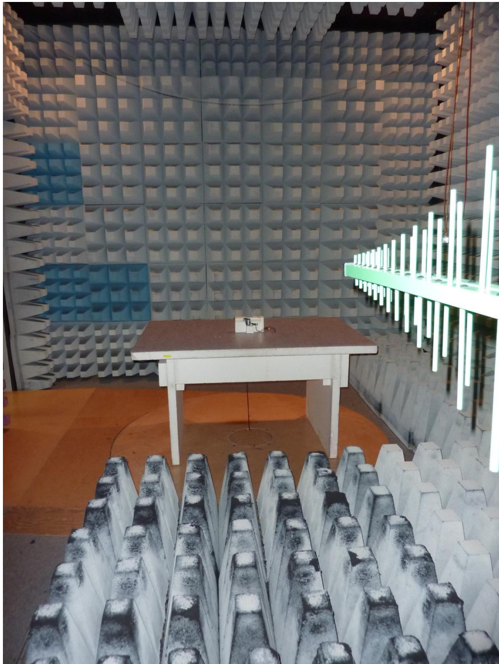
161065_1e.jpg: BT7000, test setup fully anechoic chamber
