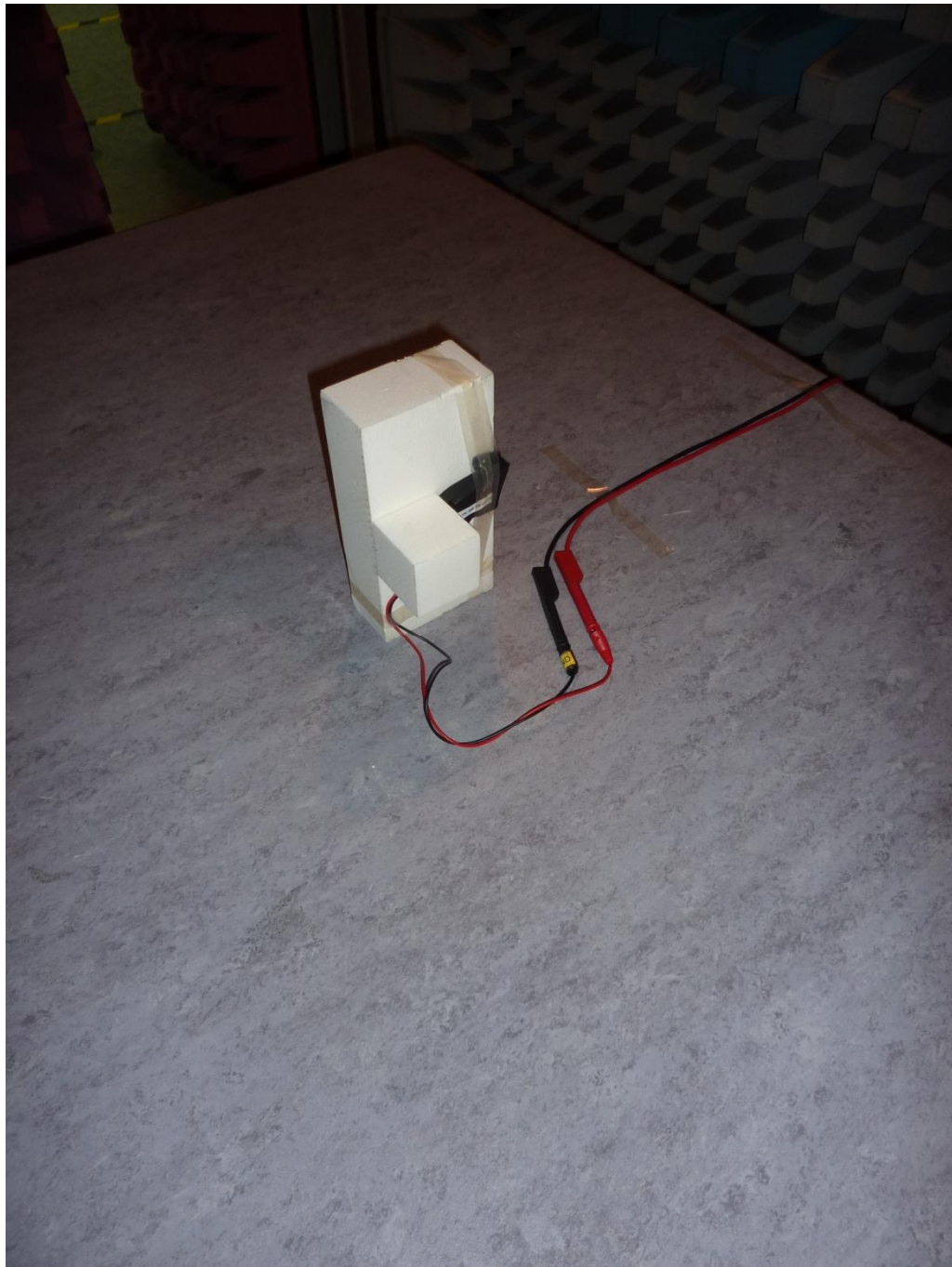
161065_1c.jpg: BT7000, test setup fully anechoic chamber (position 3)
