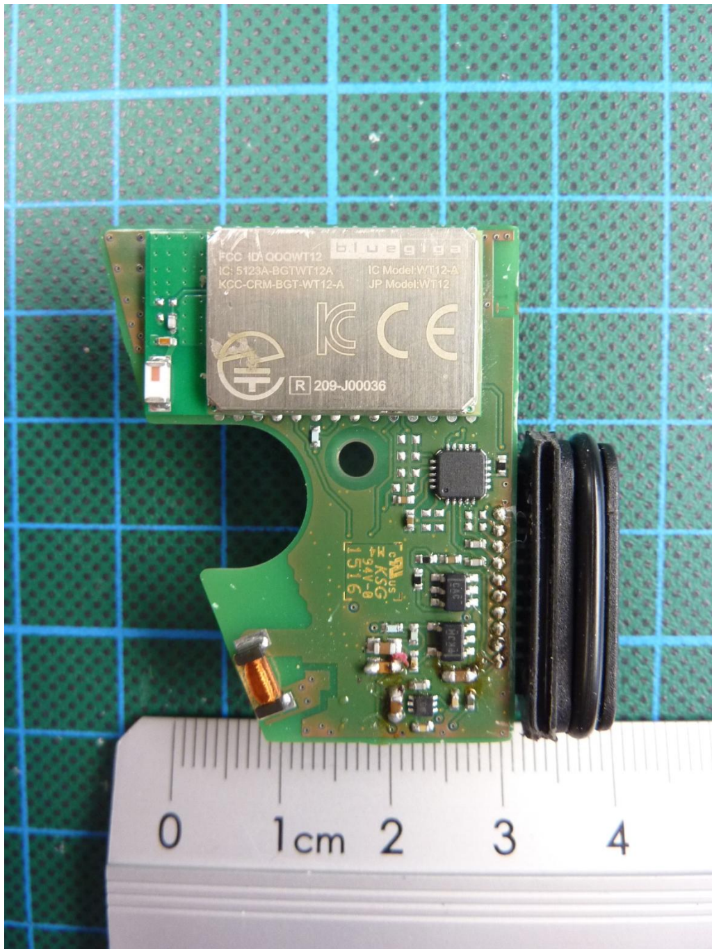
161065_107.jpg: BT7000, PCB, bottom view
