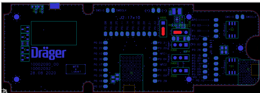
Figure 5.1-1 Test board configured for external supply
