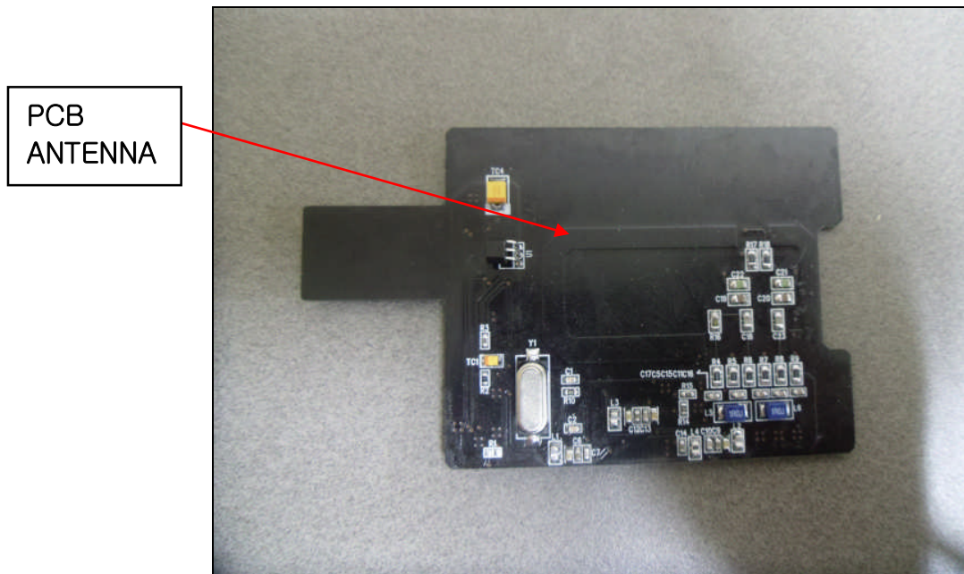
Bottom view of scan part PCB
