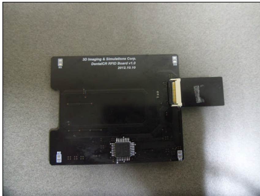
Bottom view of scan part PCB
