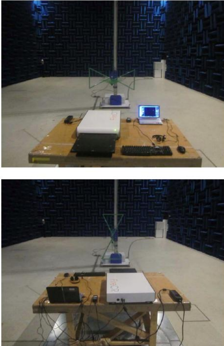
Figure 2. Photo of Radiated emission test setup:
