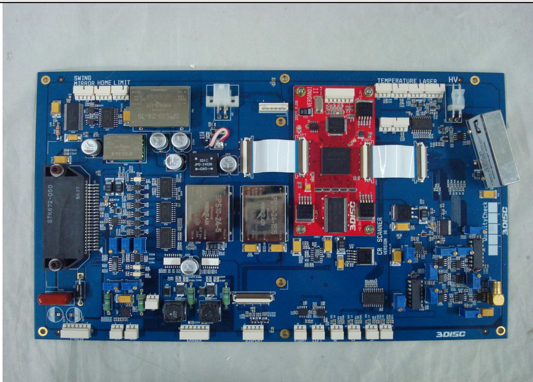
Main board front
