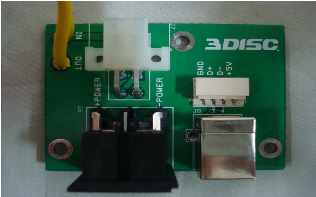
Power switch board rear
