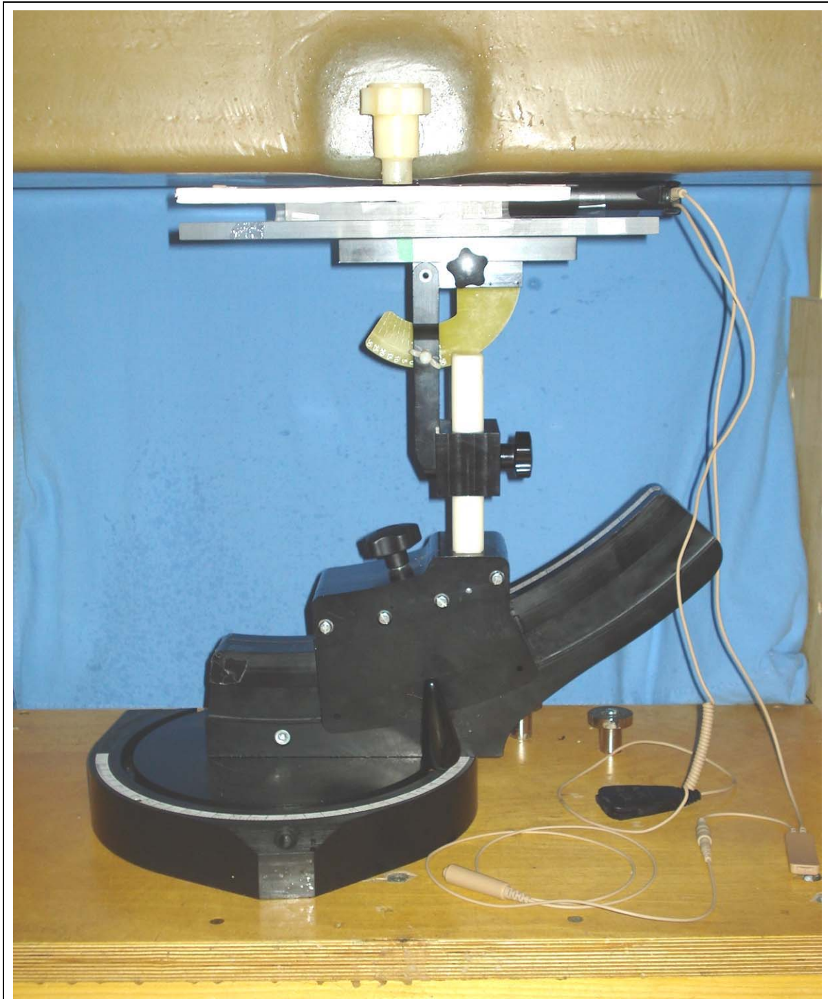
Body-worn Test Setup Configuration
