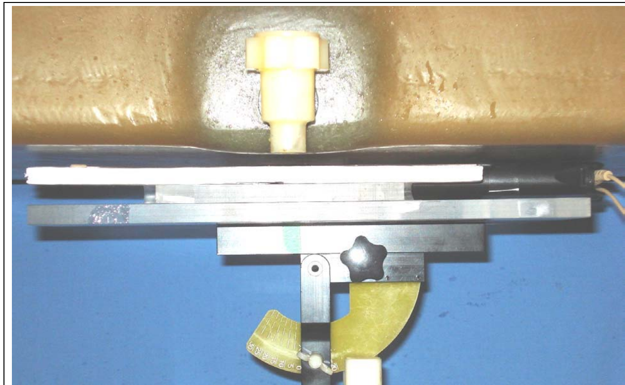
Close-up of Body-worn Test Setup Configuration
