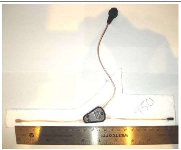
Dipole Antenna P/N: 1570.B37.006 (406.1-450 MHz)
