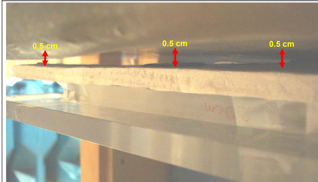
0.5 cm Separation Distance between Dipole Antenna and Planar Phantom
