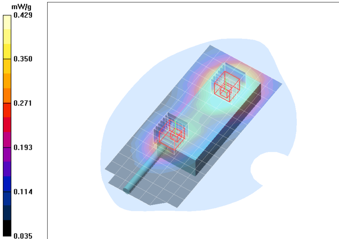
Fig. 18: SAR distribution for Tetra, 868.9875 MHz, body worn configuration, with shoulder belt case (July 31, 2012; Ambient Temperature: 22.7° C; Liquid Temperature: 22.4° C).
