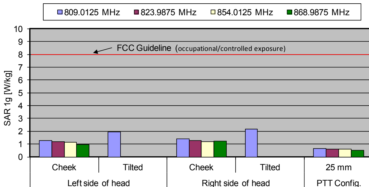
Fig. 8: The measured head SAR values for the Selex Elsag S.p.A. PUMA T3 plus for TETRA in head and PTT configuration, in comparison to the FCC exposure limit.
