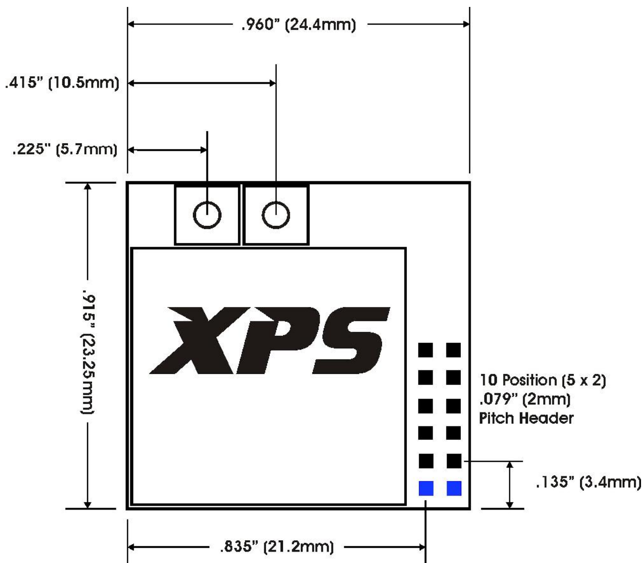
Figure 3-1. DivBee™ Top View Mechanical Drawing (blue connections optional)
