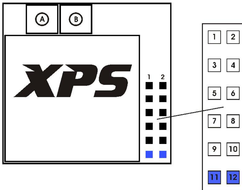
Figure 3-3. DivBee™ Pinout, Refer to Table 3-4 for pin descriptions
