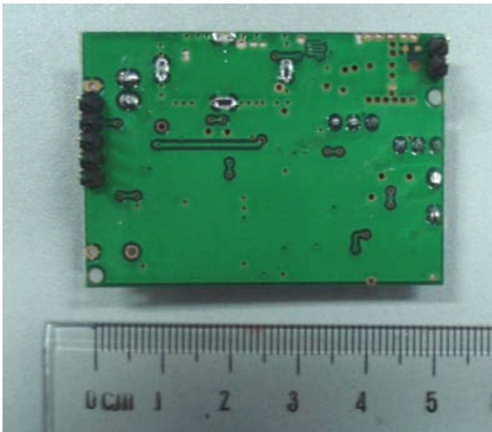
Receiver Board Back View
