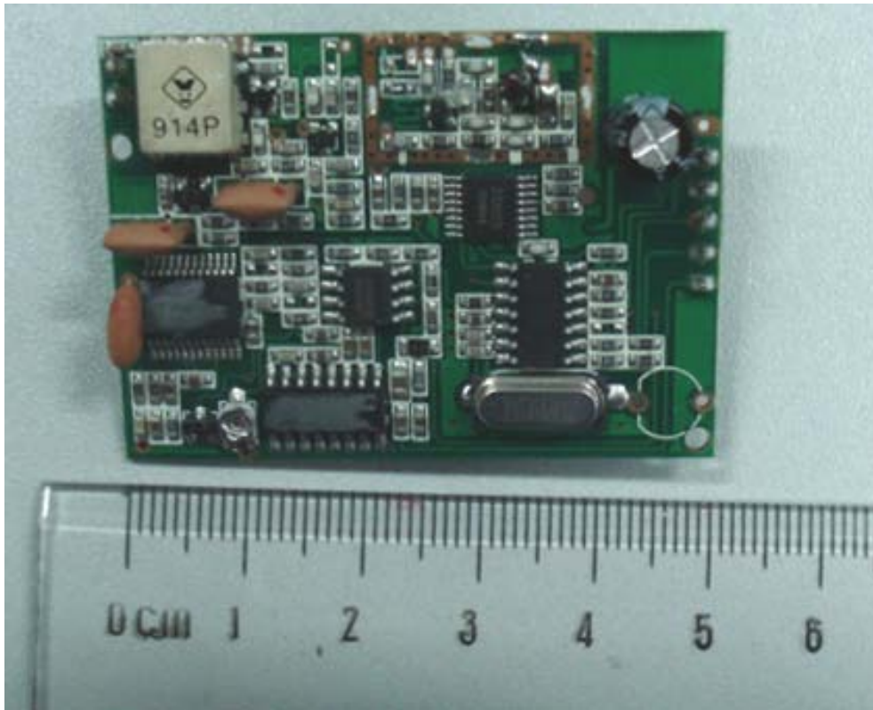
Receiver Board Front View
