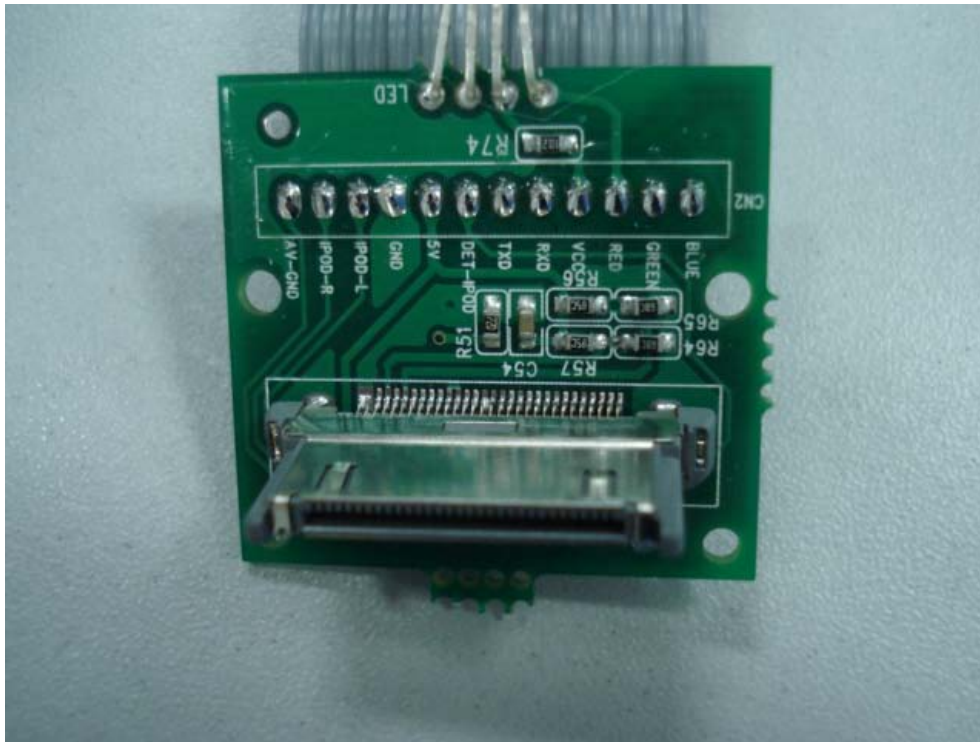
IPOD Board Front View
