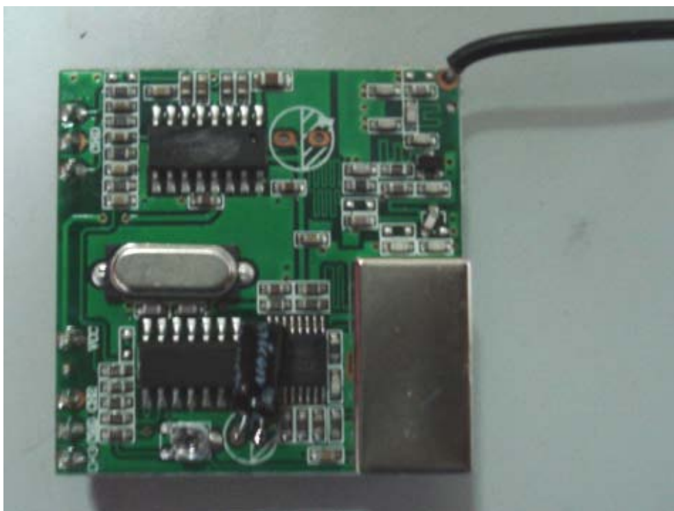
Transmit Board Front View-1
