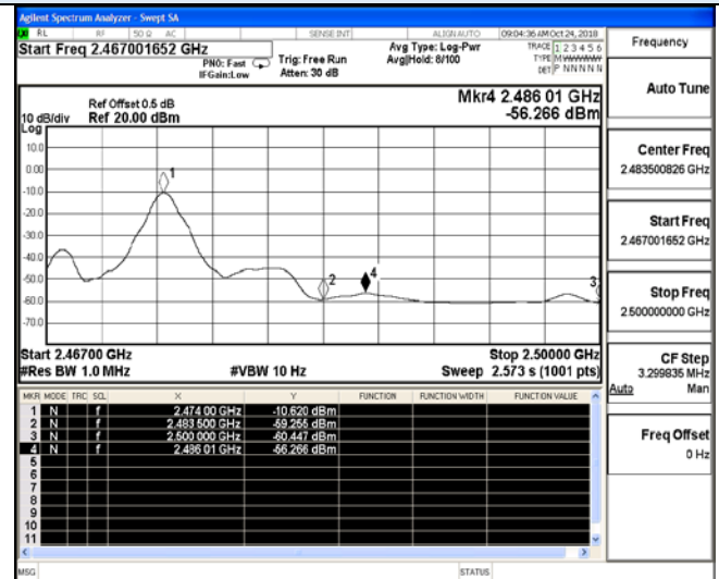
2474 MHz – Average
