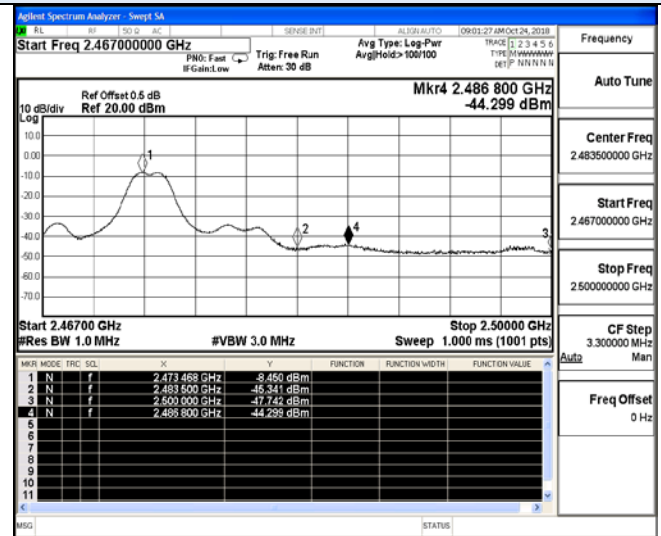
2474 MHz – Peak
