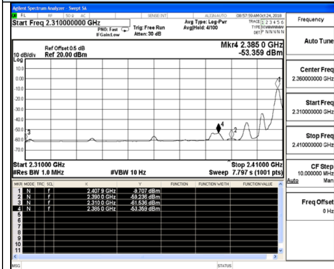
2408 MHz – Average
