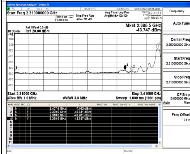
2408 MHz – Peak
