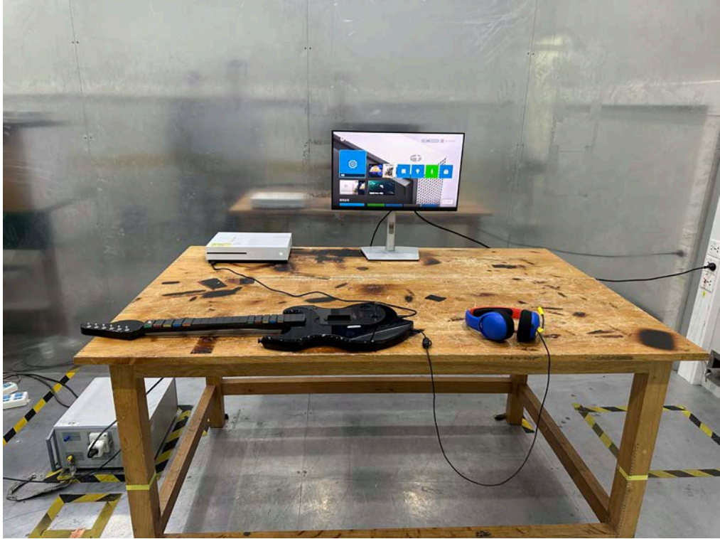
Conduction Setup photo
