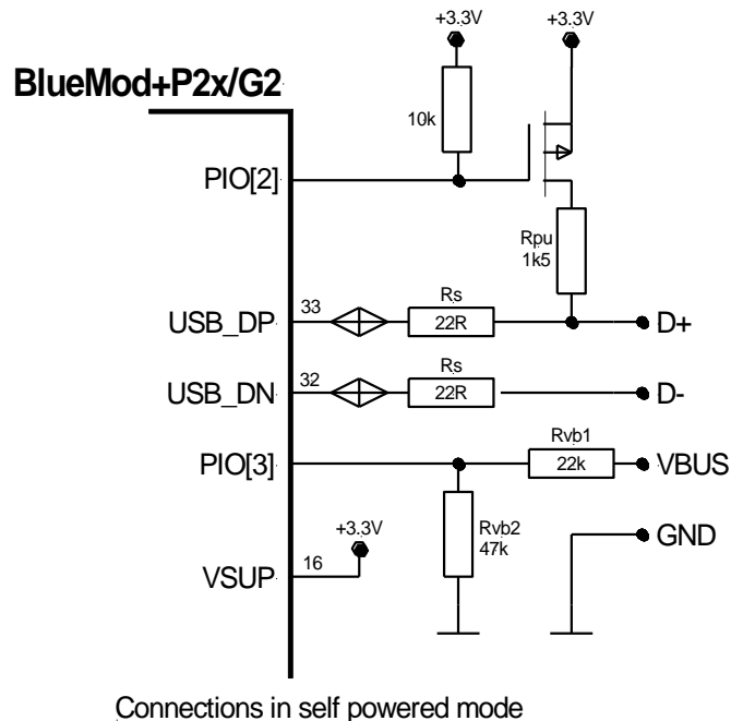
Figure 3.3 BlueMod+P2x/G2 USB Self-Powered Mode
