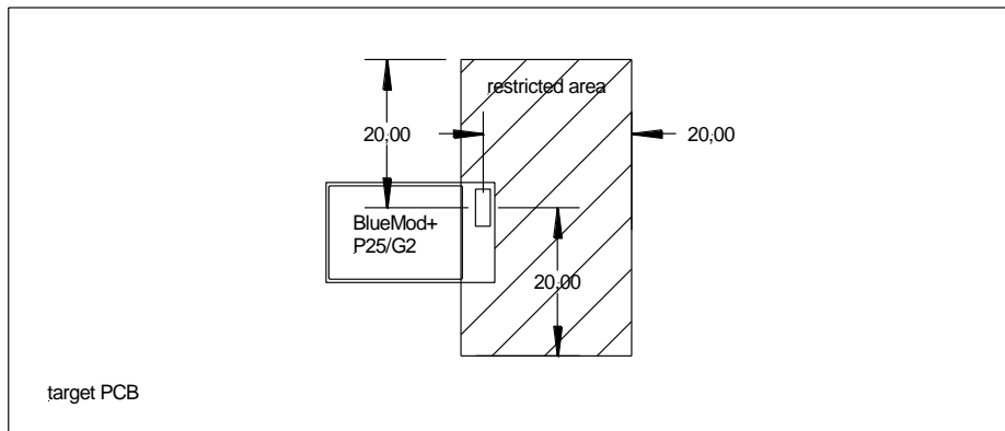
Figure 6.10 acceptable, but not optimal placement (not in scale, dimension in mm)
