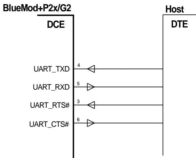
Figure 3.1 BlueMod+P2x/G2 Serial Interface
