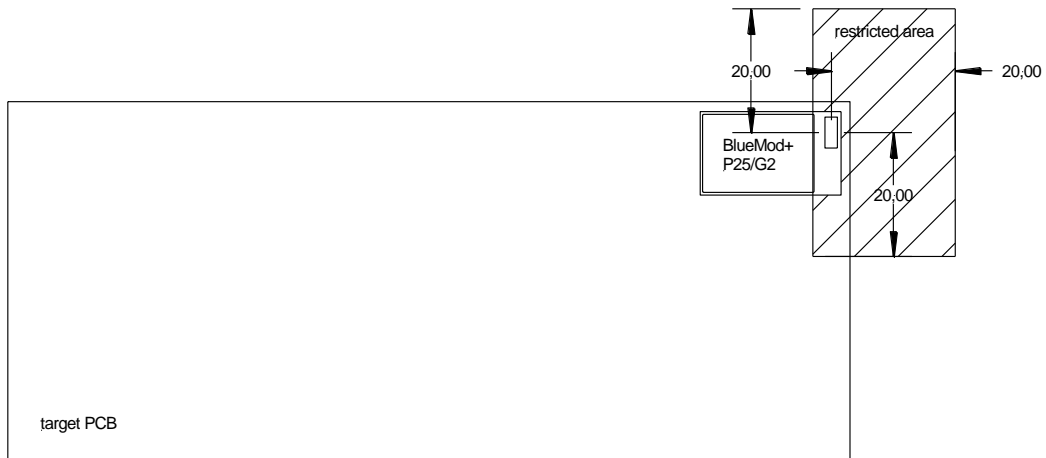
Figure 6.8 Optimal placement (not in scale, dimension in mm)
