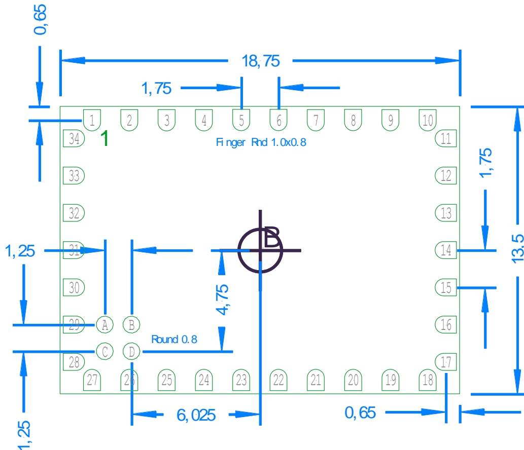
Figure 6.3 BlueMod+P24/G2 Recommended Land pattern (Top-View, not in scale, dimension in mm)
