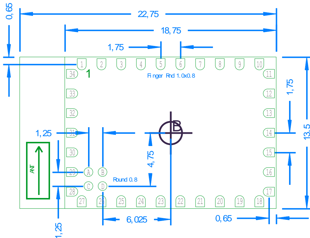
Figure 6.4 BlueMod+P25/G2 Recommended Land pattern (Top-View, not in scale, dimension in mm)
