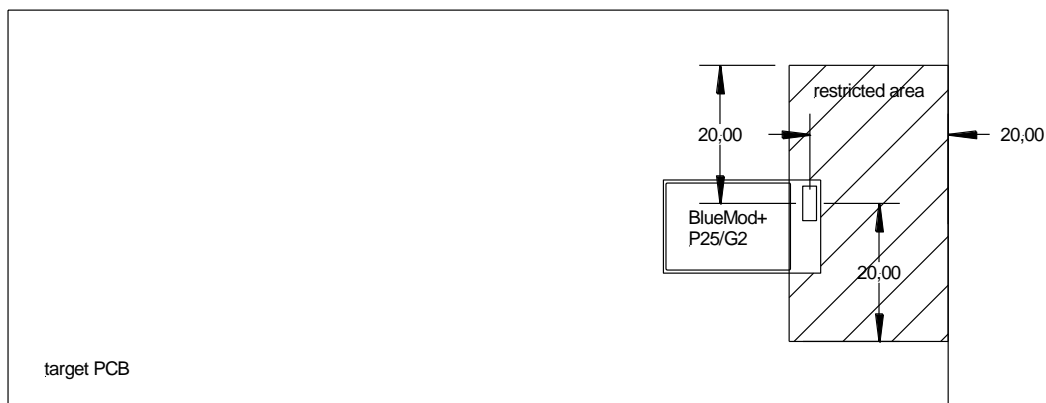
Figure 6.9 recommendable placement (not in scale, dimension in mm)
