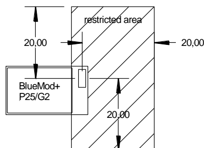
Figure 6.7 BlueMod+P25/G2 Recommended Restricted Area(not in scale, dimension in mm)
