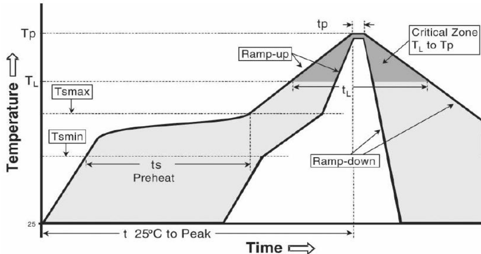
Figure 6.11 Soldering Temperature-Time Profile (for reflow soldering)
