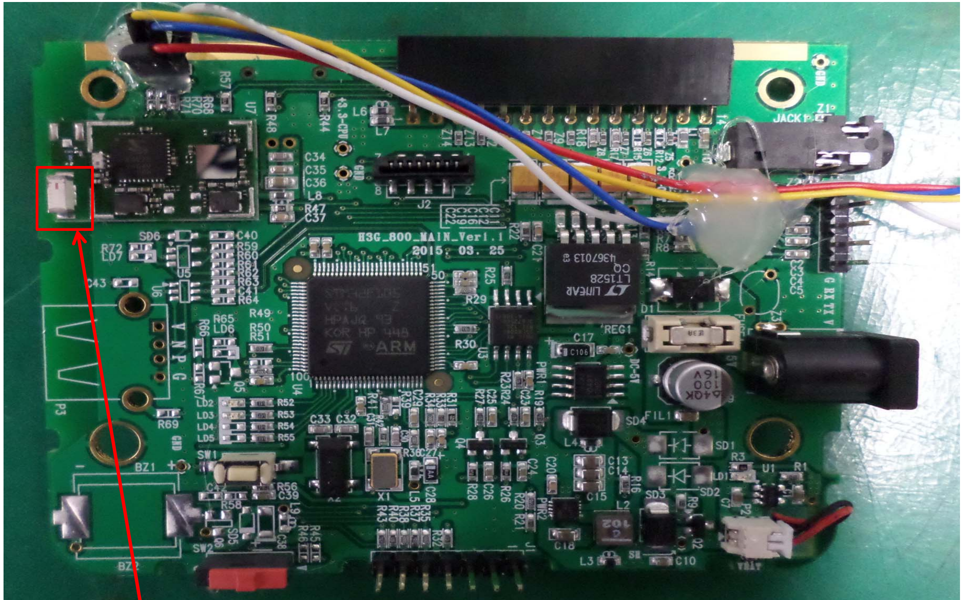
BT Antenna
