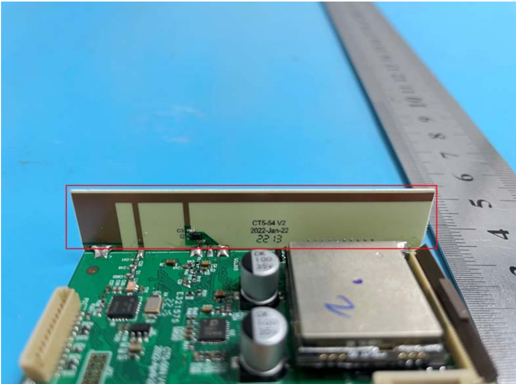
Antenna-CRMX(Only reception function)
