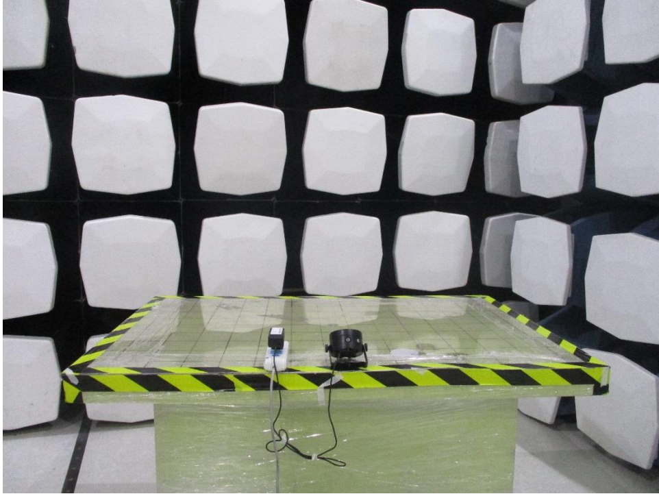
Below 1GHz
