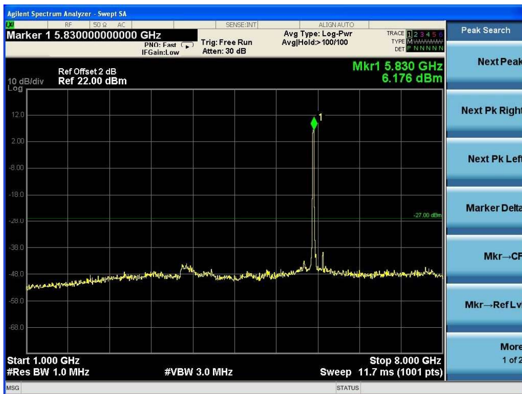
(Plot 4.9.3 C4: Channel 165: 5825MHz @ 802.11a)
