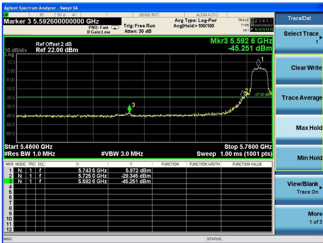
(Plot 4.9.4 A1: Channel 149: 5745MHz @ 802.11n HT20)
