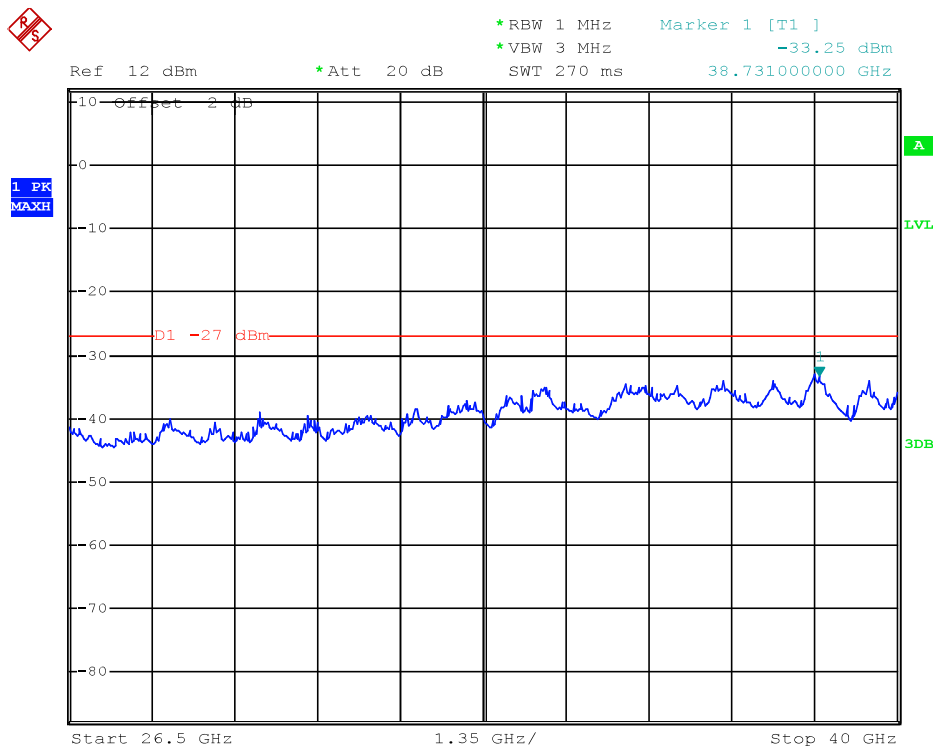
(Plot 4.9.3 B7: Channel 157: 5785MHz @ 802.11a)
