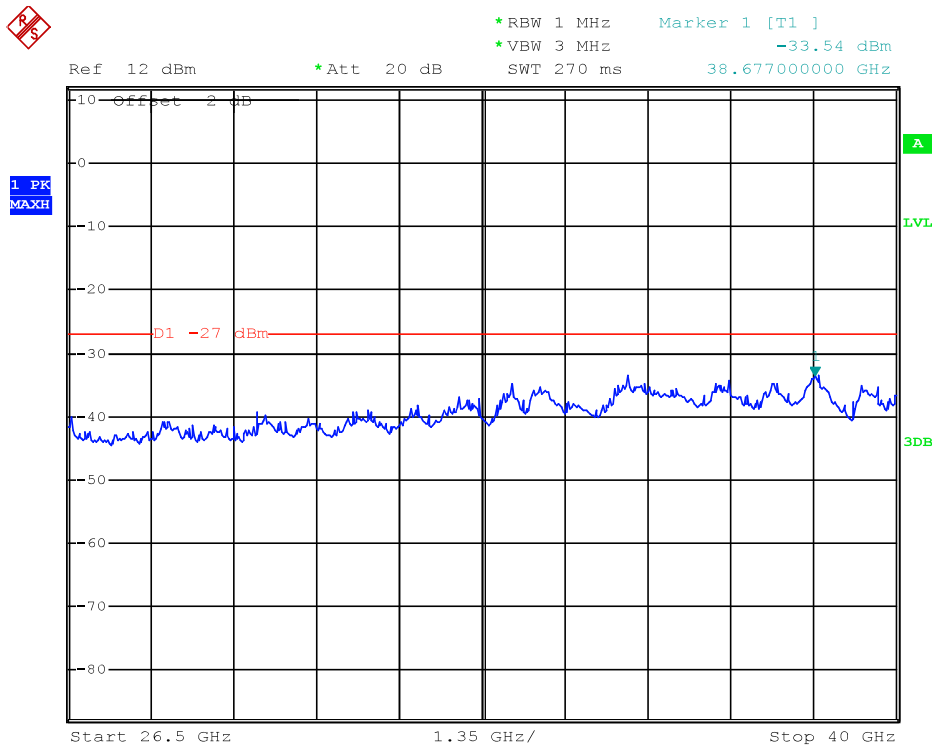
(Plot 4.9.4 A7: Channel 149: 5745MHz @ 802.11n HT20)
