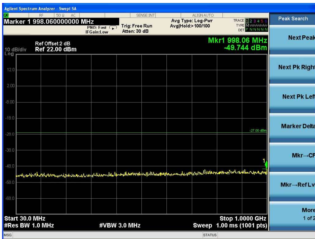
(Plot 4.9.3 C3: Channel 165: 5825MHz @ 802.11a)
