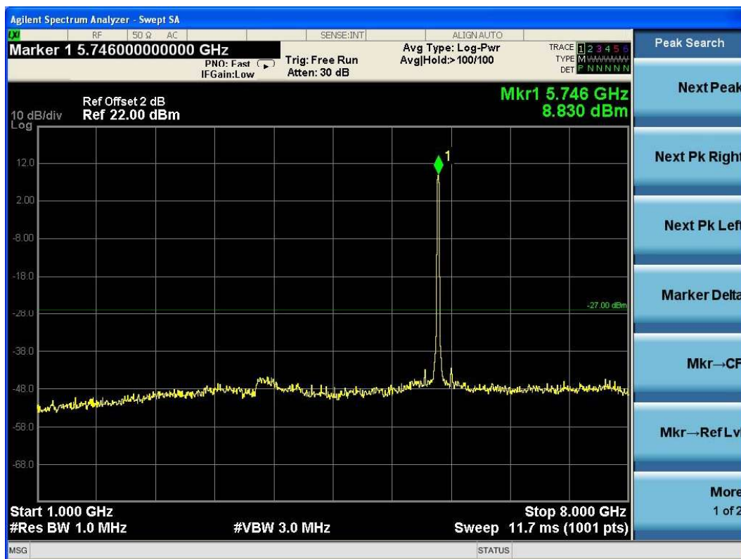
(Plot 4.9.3 A4: Channel 149: 5745MHz @ 802.11a)
