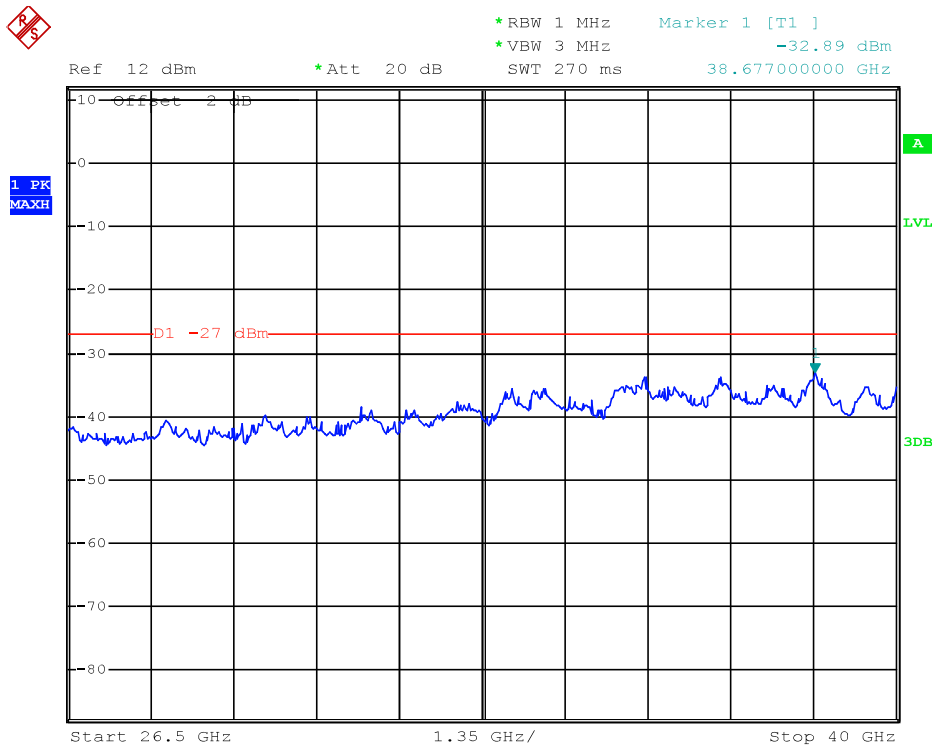
(Plot 4.9.4 C7: Channel 165: 5825MHz @ 802.11n HT20)
