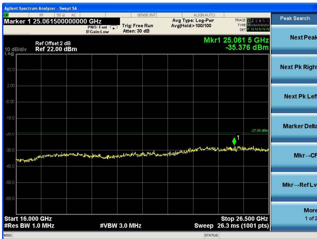
(Plot 4.9.3 A6: Channel 149: 5745MHz @ 802.11a)
