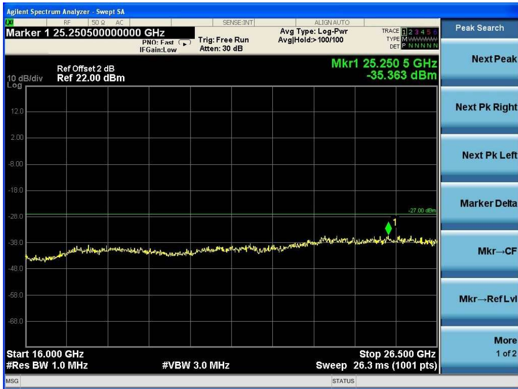
(Plot 4.9.2 C6: Channel 48: 5240MHz @ 802.11n HT20)
