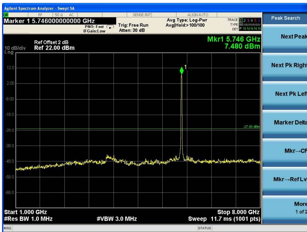
(Plot 4.9.4 A4: Channel 149: 5745MHz @ 802.11n HT20)
