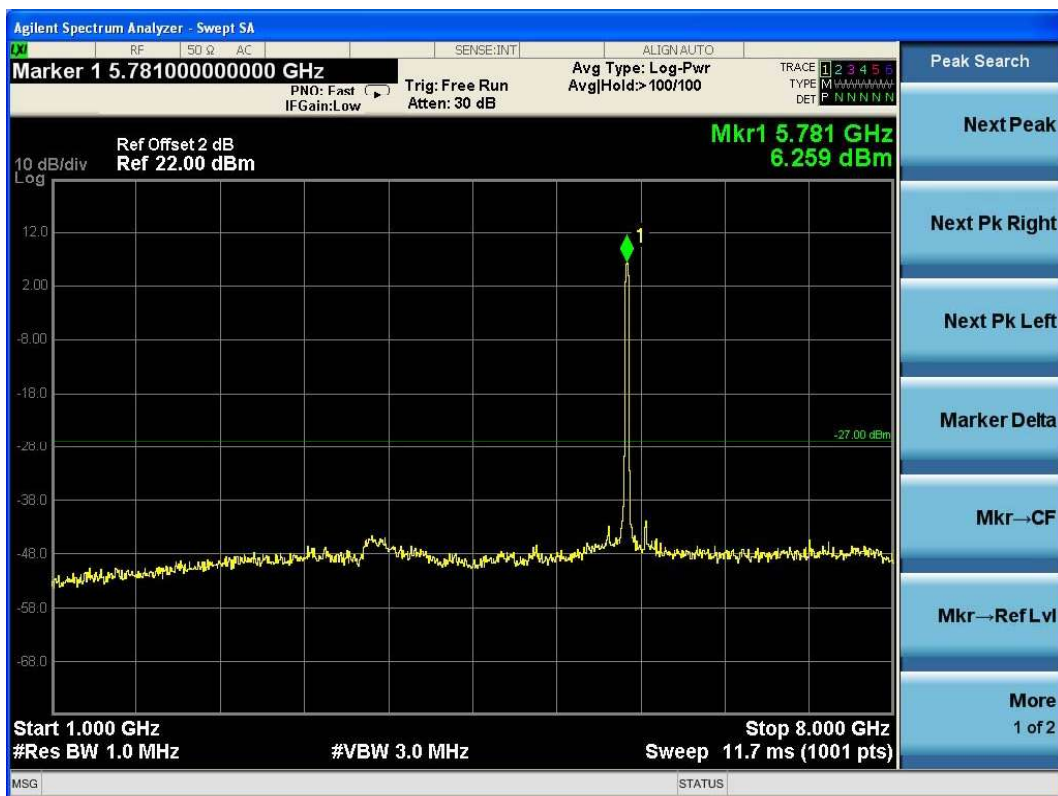
(Plot 4.9.4 B4: Channel 157: 5785MHz @ 802.11n HT20)
