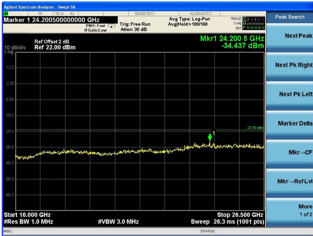
(Plot 4.9.4 A6: Channel 149: 5745MHz @ 802.11n HT20)
