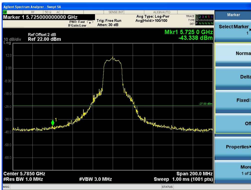
(Plot 4.9.4 B1: Channel 157: 5785MHz @ 802.11n HT20)
