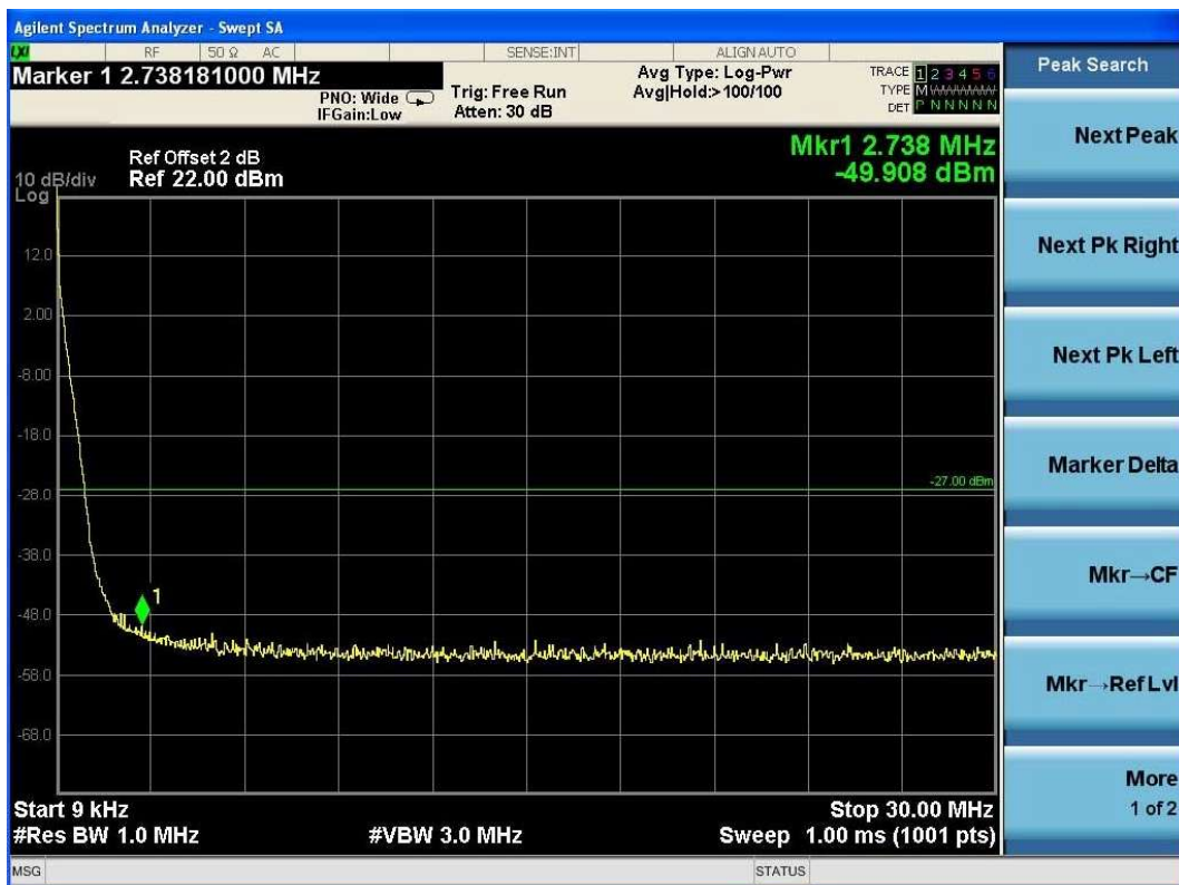
(Plot 4.9.3 A2: Channel 149: 5745MHz @ 802.11a)
