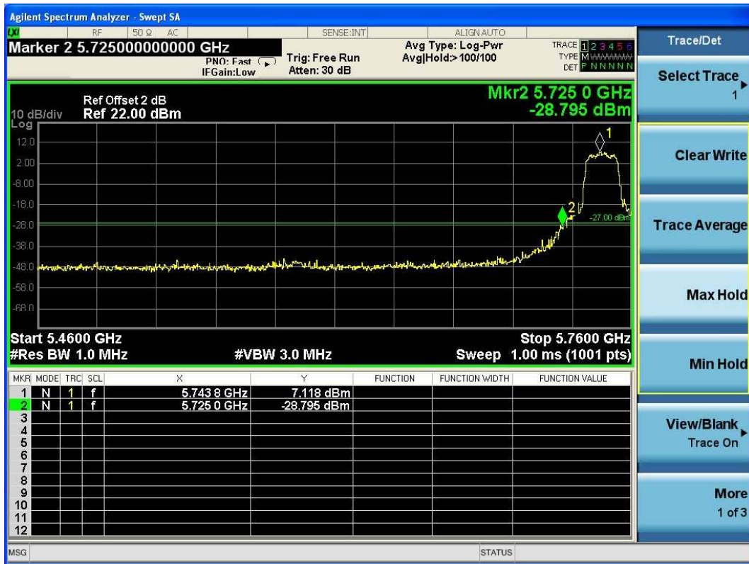
(Plot 4.9.3 A1: Channel 149: 5745MHz @ 802.11a)
