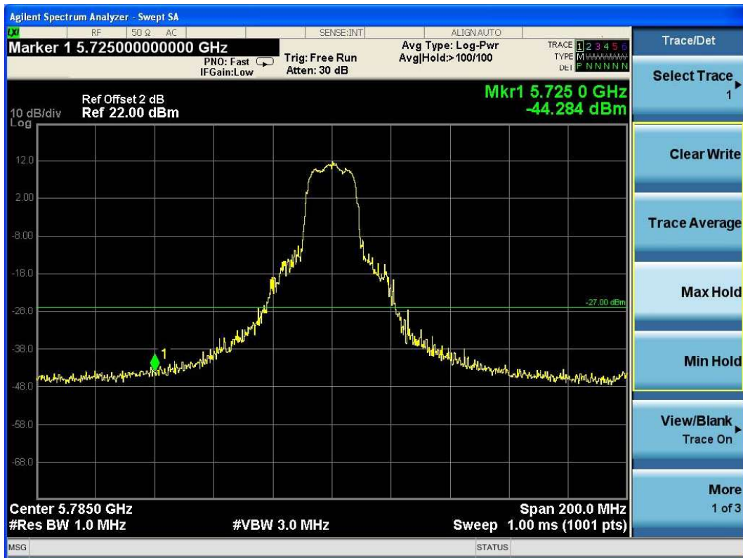
(Plot 4.9.3 B1: Channel 157: 5785MHz @ 802.11a)
