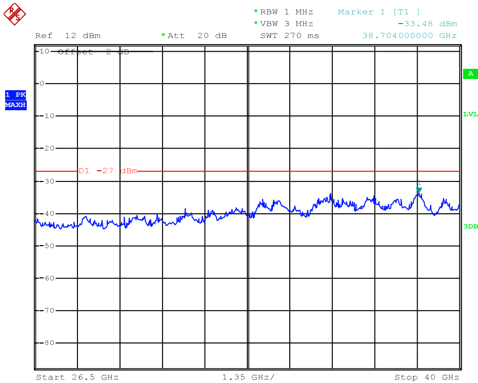
(Plot 4.9.4 B7: Channel 157: 5785MHz @ 802.11n HT20)
