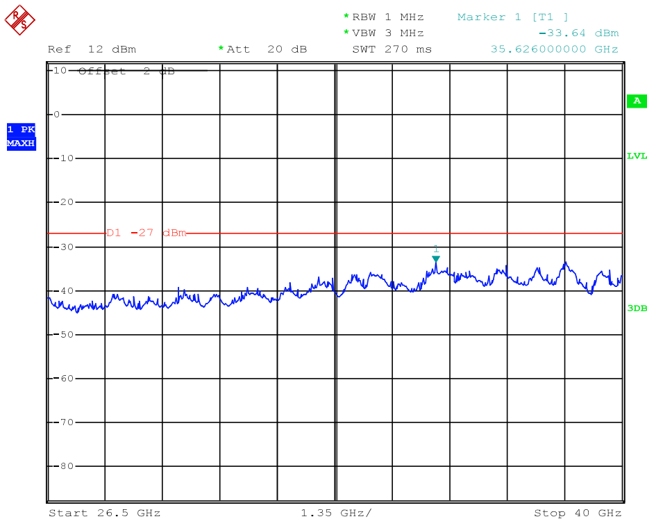
(Plot 4.9.3 C7: Channel 165: 5825MHz @ 802.11a)
