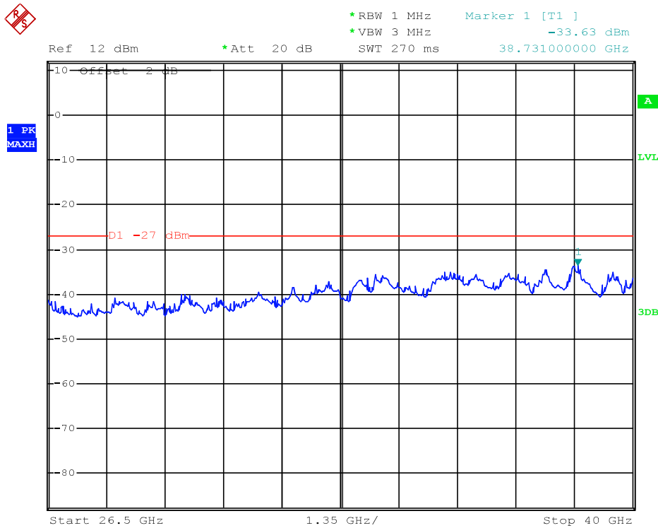
(Plot 4.9.3 A7: Channel 149: 5745MHz @ 802.11a)
