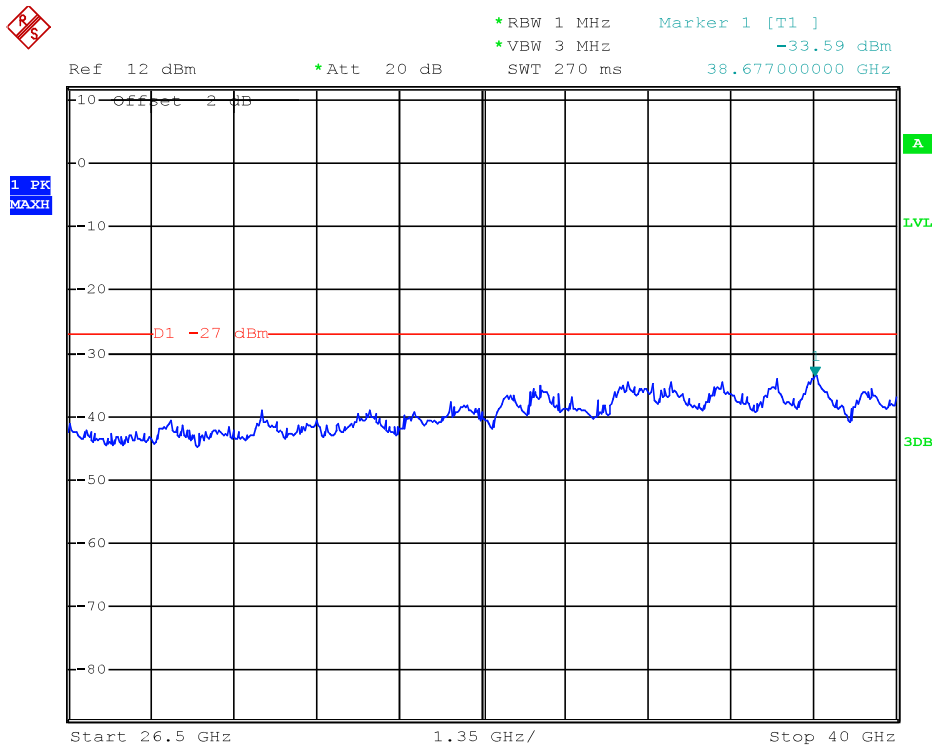
(Plot 4.9.2 C7: Channel 48: 5240MHz @ 802.11n HT20)
