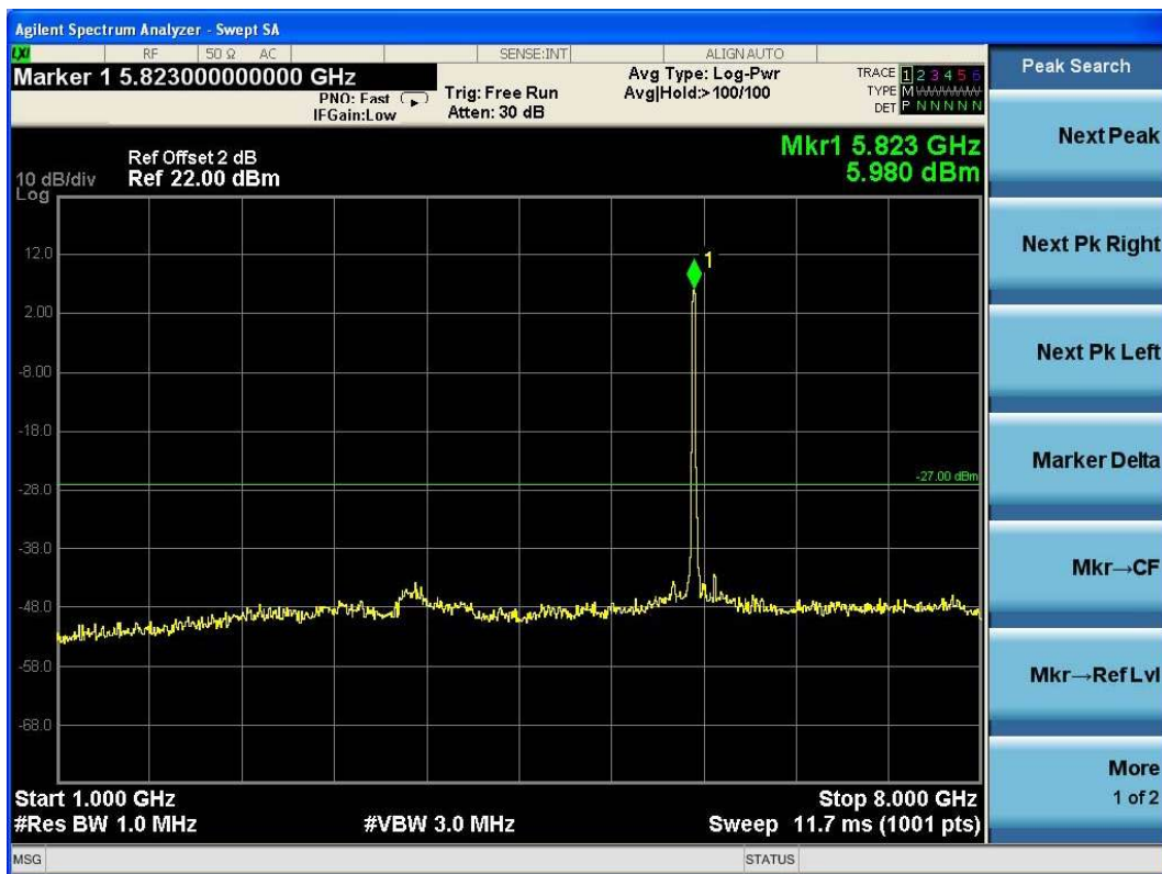
(Plot 4.9.4 C4: Channel 165: 5825MHz @ 802.11n HT20)
