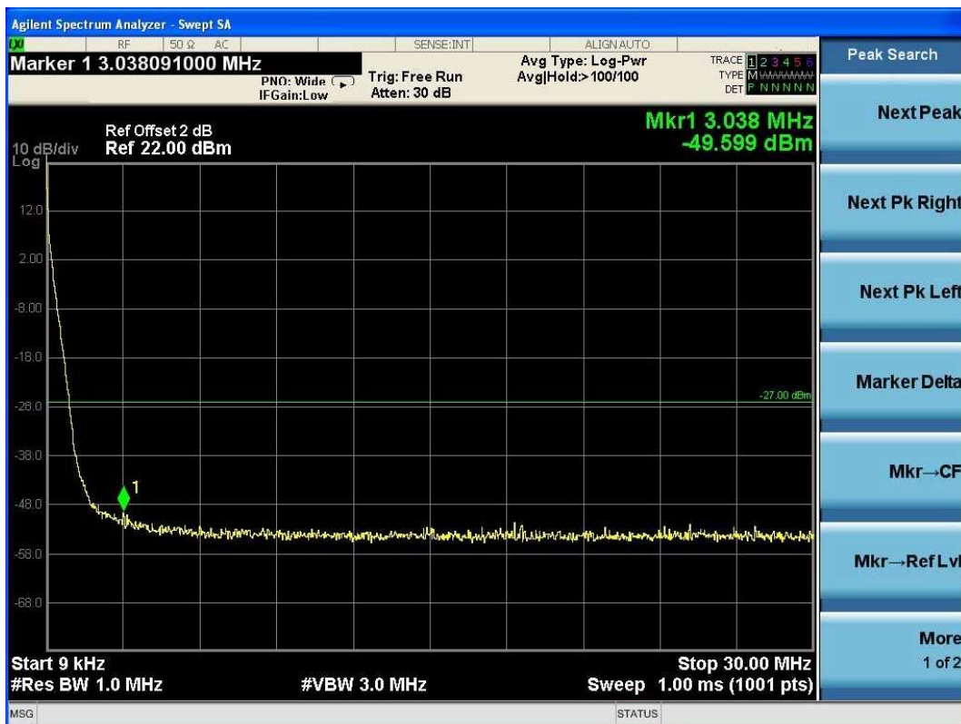
(Plot 4.9.3 C2: Channel 165: 5825MHz @ 802.11a)
