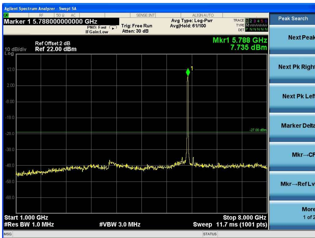
(Plot 4.9.3 B4: Channel 157: 5785MHz @ 802.11a)
