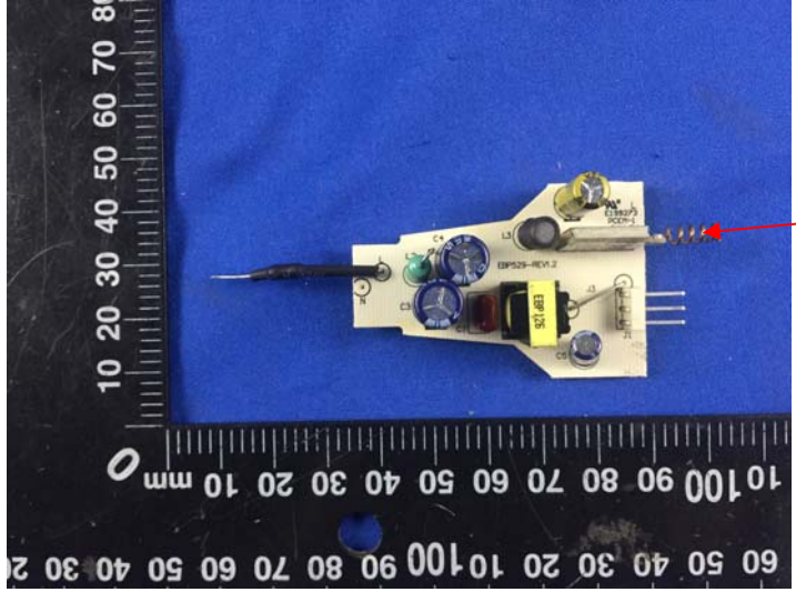
WIFI Antenna
