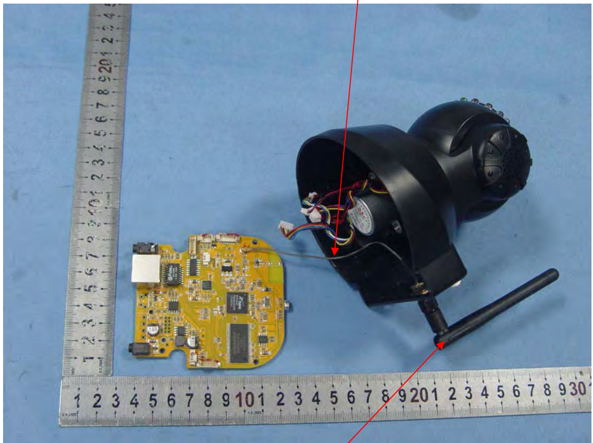
RP-SMA antenna
