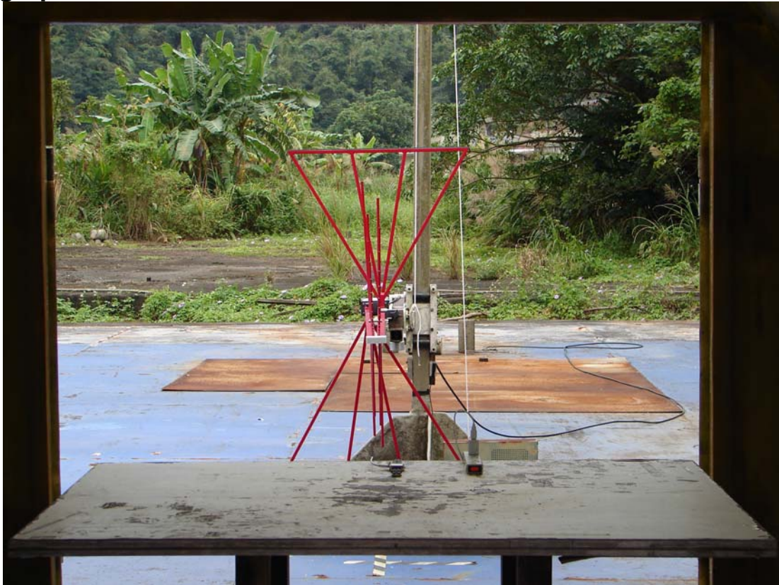
Front View of The Test Configuration (USB charge)
