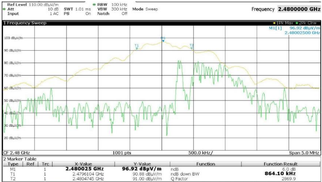
Channel 2480 MHz
