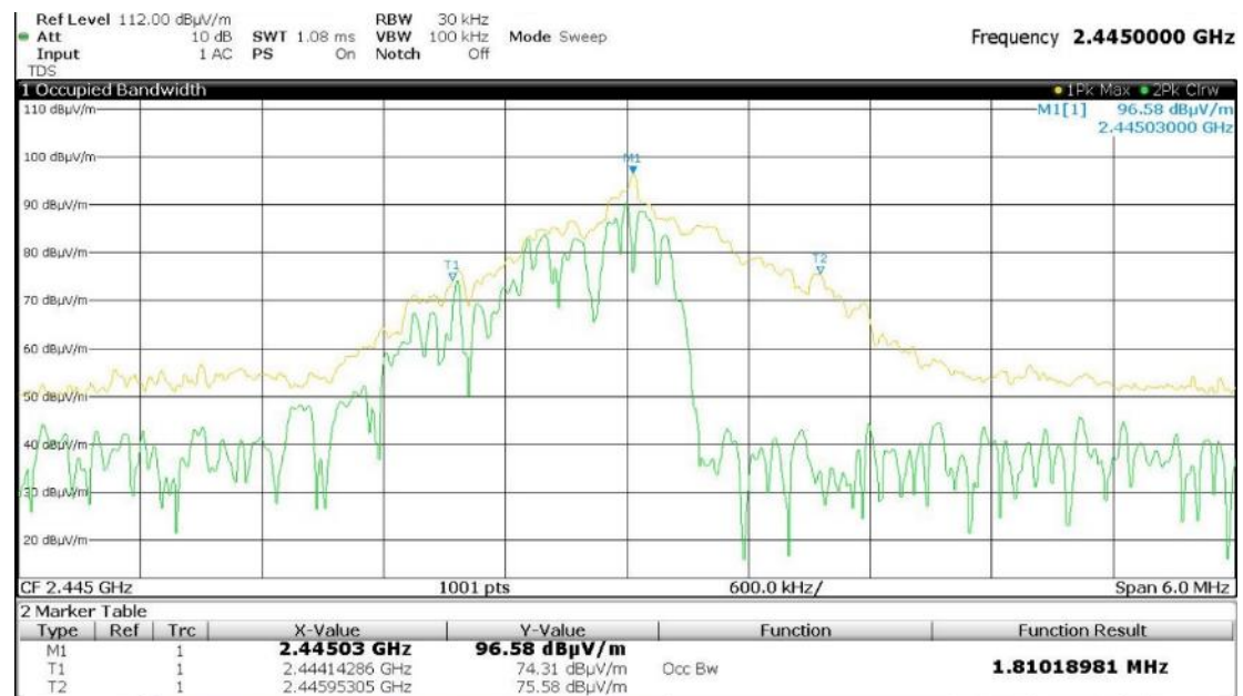
Channel 2445 MHz
