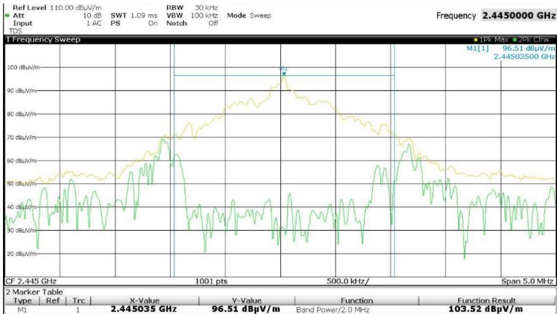
Channel 2445 MHz
