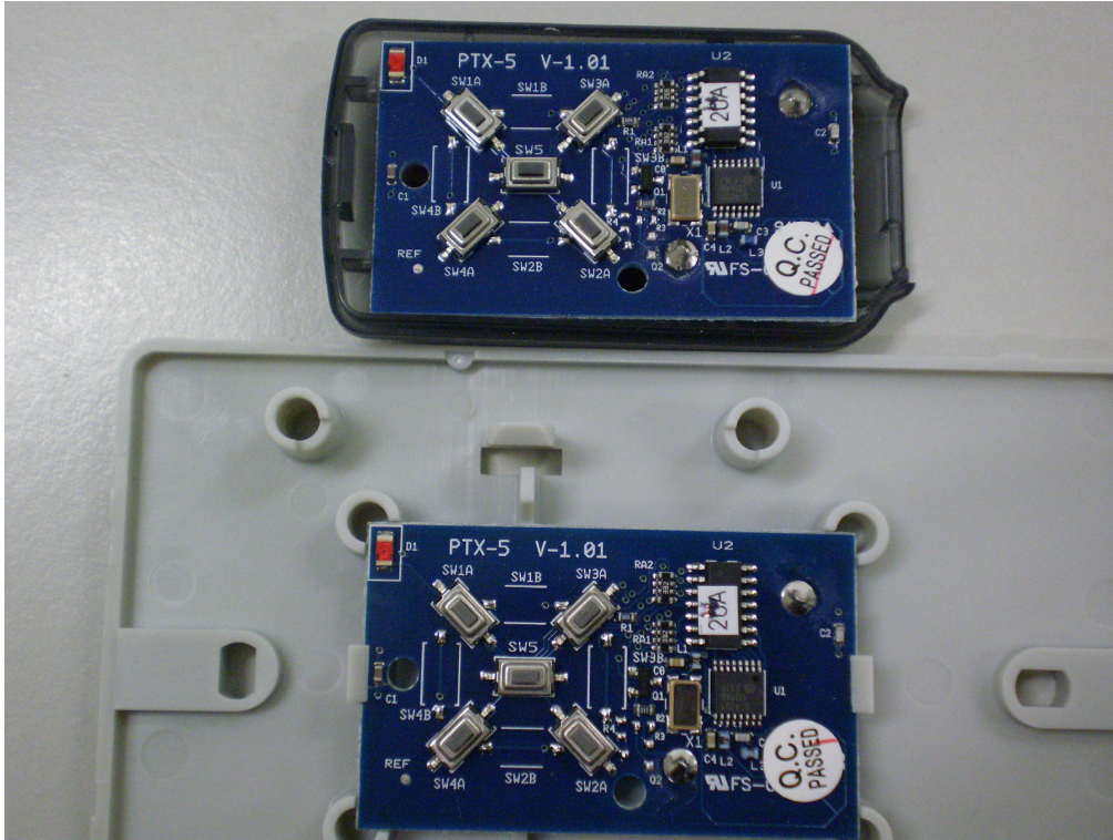
Internal Photos – PTX-5V1 and WTX-4
