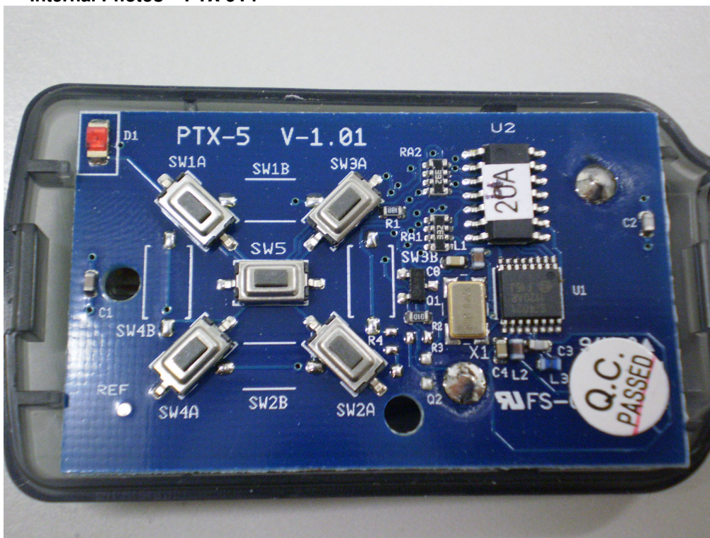
Internal Photos – PTX-5V1
