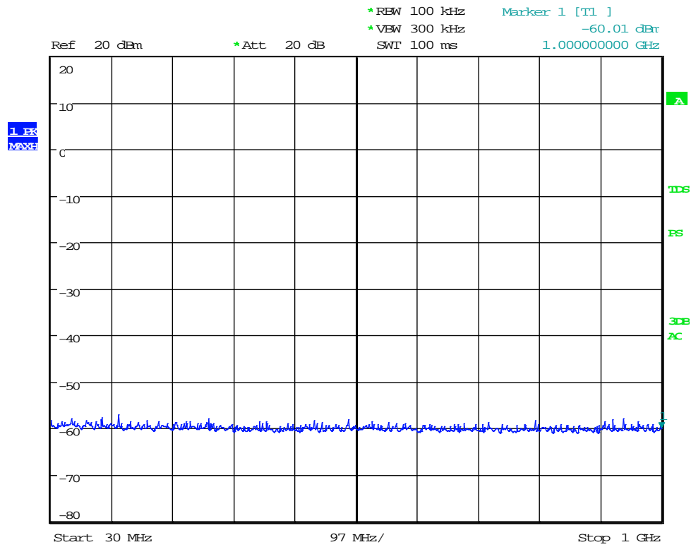
Graph 6-3: Conducted Spurious Emissions, 30 – 1000 MHz IEEE 802.11n-HT20 (MCS0), Channel 11 (2462 MHz)
