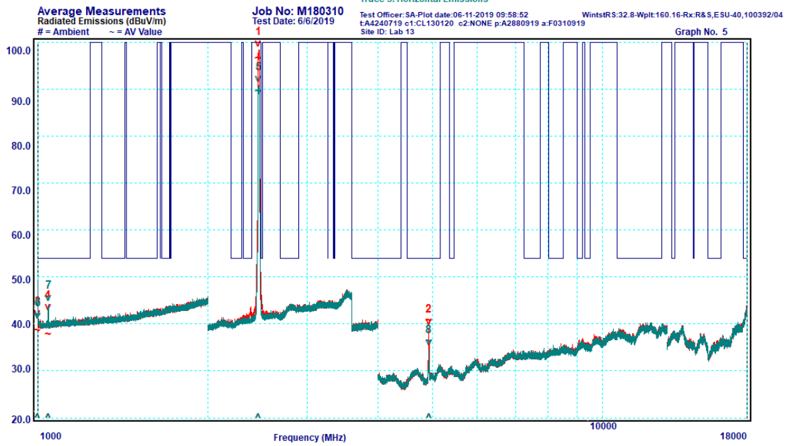
Graph 6-6: Radiated Spurious Emissions - Average, 1000 MHz – 18000 MHz IEEE 802.11n-HT20 (MCS0), Channel 11 (2462 MHz)
