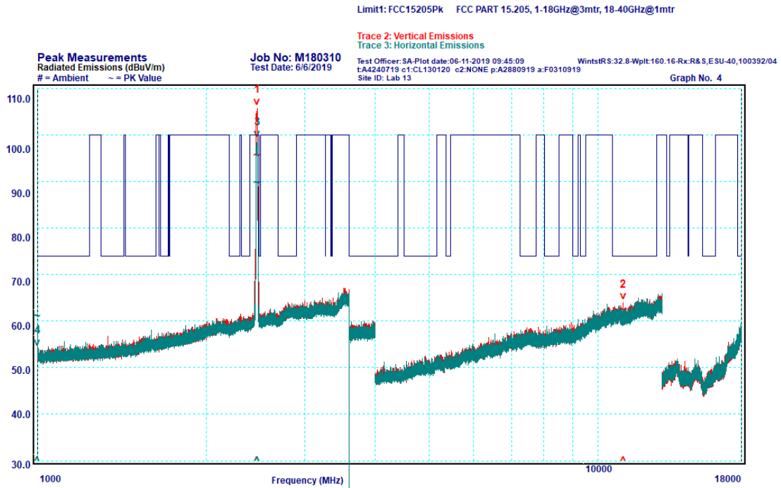
Graph 6-5: Radiated Spurious Emissions - Peak, 1000 MHz – 18000 MHz IEEE 802.11n-HT20 (MCS0), Channel 11 (2462 MHz)
