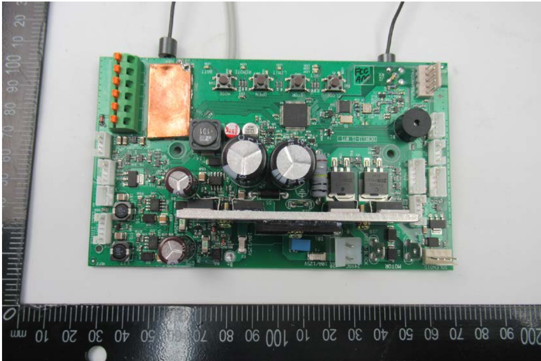
902 – 928 MHz Transceiver
