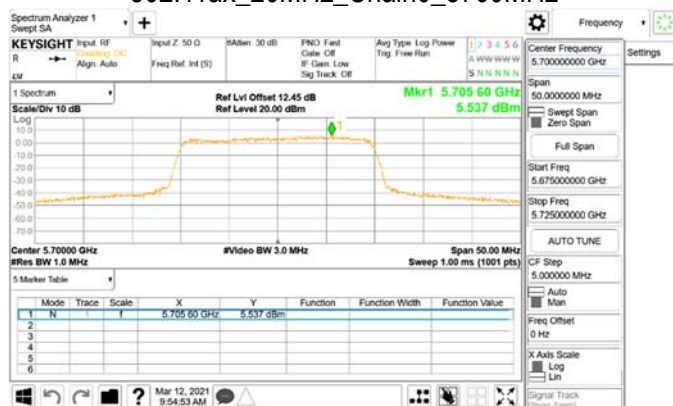
802.11ax_20MHz_Chain0_5700MHz_RU106_54
