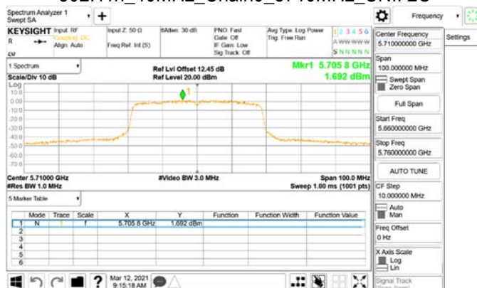
802.11n_40MHz_Chain0_5710MHz_UNII 3
