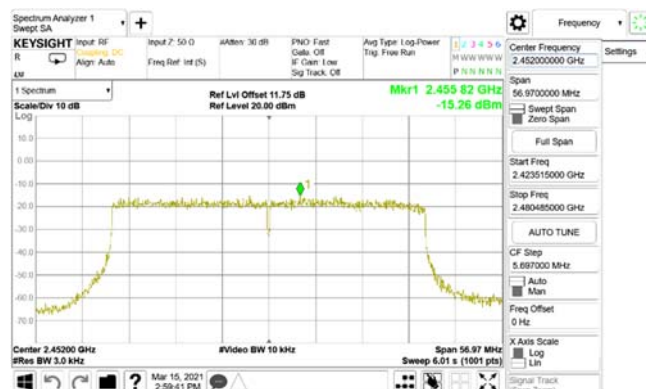
Power Density_802.11ax_40MHz_Chain0_2452MHz_RU242_62
