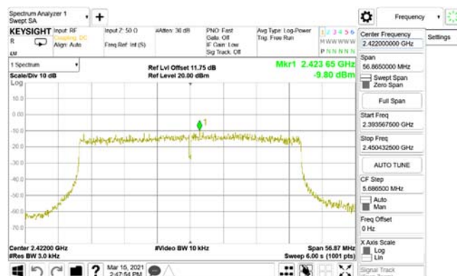
Power Density_802.11ax_40MHz_Chain1_2422MHz
