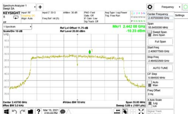
Power Density_802.11ax_40MHz_Chain1_2437MHz
