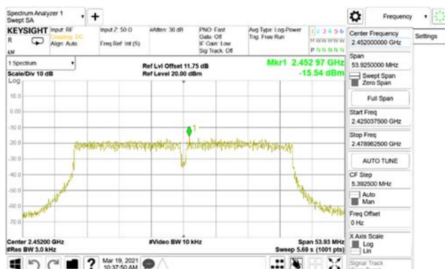
Power Density_802.11n_40MHz_Chain0_2452MHz
