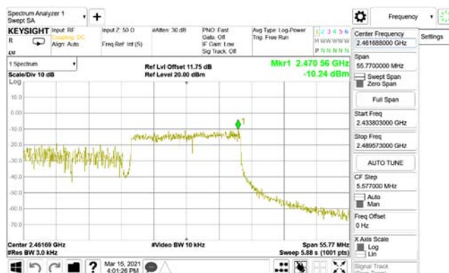
Power Density_802.11ax_40MHz_Chain1_2452MHz_RU242_62
