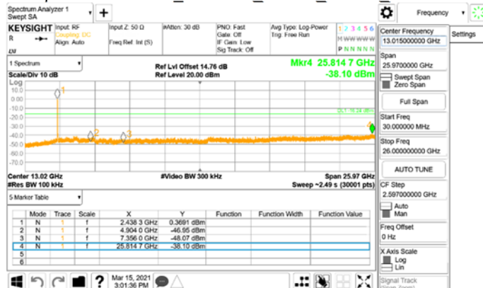
Spurious Emission_802.11ax_40MHz_Chain0_2452MHz
