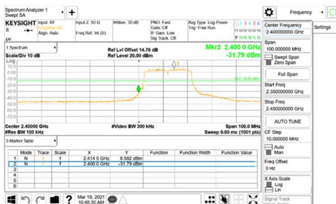
Bandedge_802.11ax_20MHz_Chain0_2412MHz
