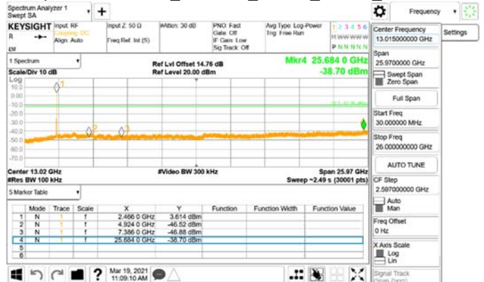
Spurious Emission_802.11ax_20MHz_Chain0_2462MHz
