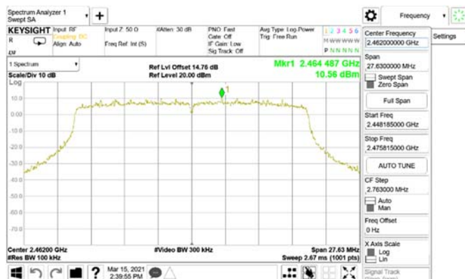
Reference Level_802.11ax_20MHz_Chain0_2462MHz
