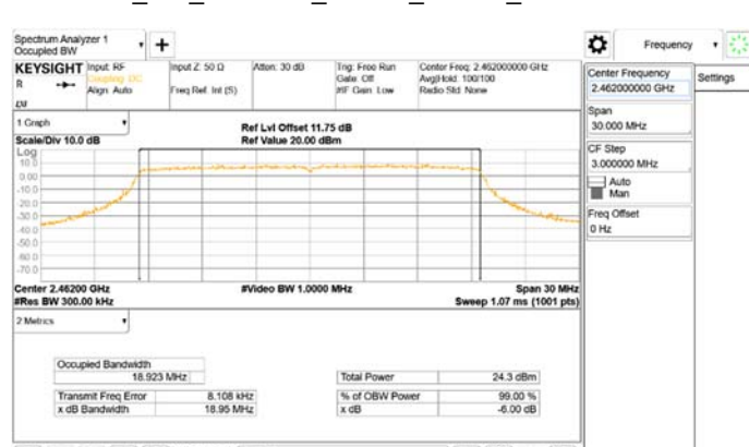
99% BW_802.11ax_20MHz_Chain1_2462MHz
