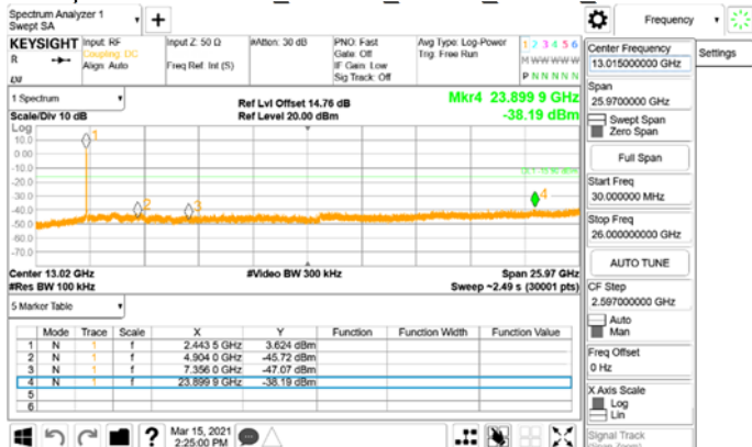
Spurious Emission_802.11n_40MHz_Chain0_2452MHz
