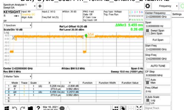
Duty Cycle_802.11ax_40MHz_Chain0_2422MHz
