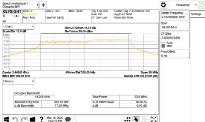
6dB_BW_802.11ax_20MHz_Chain0_2462MHz_RU26_8
