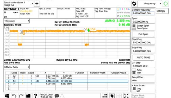
Duty Cycle_802.11ax_40MHz_Chain0_2422MHz
