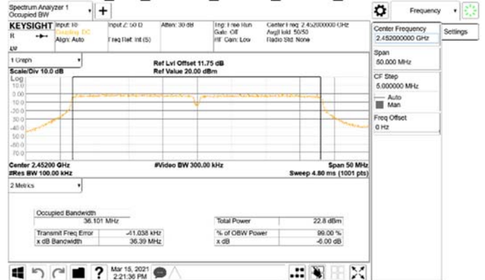
6dB_BW_802.11n_40MHz_Chain1_2452MHz
