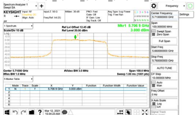
802.11ax_40MHz_Chain1_5710MHz_UNII 3
