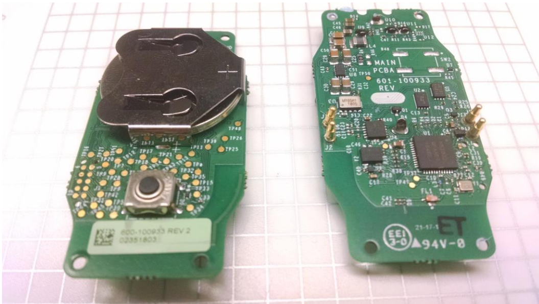
EP04014 PCBA (both sides)
