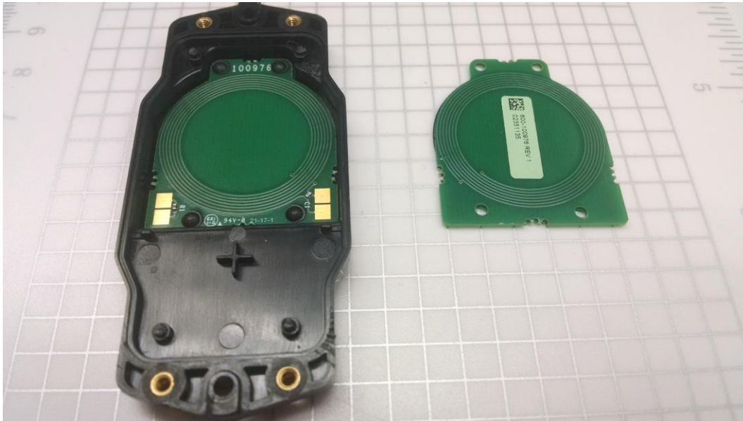
EP04013 PCBA (both sides)
