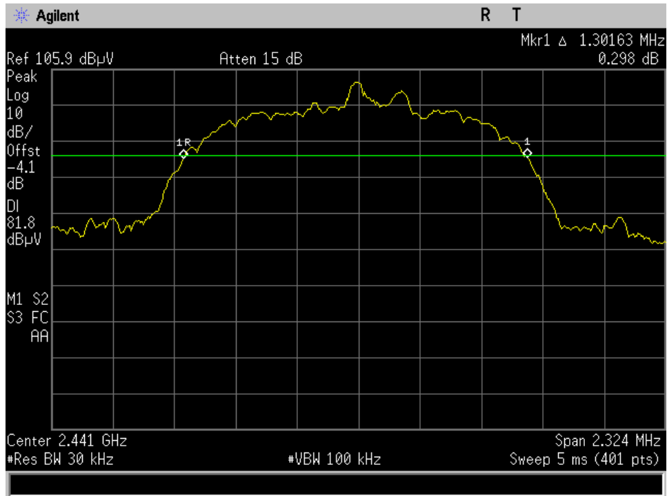
mid ch DH5 20dB and 99%
