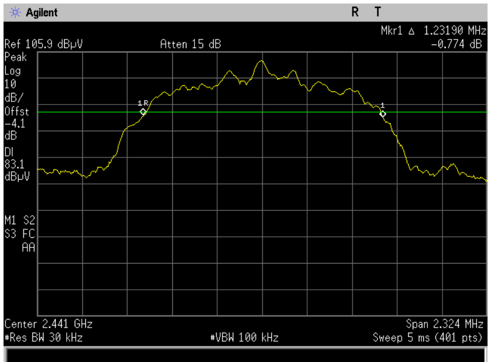
mid ch DH1 20dB and 99%
