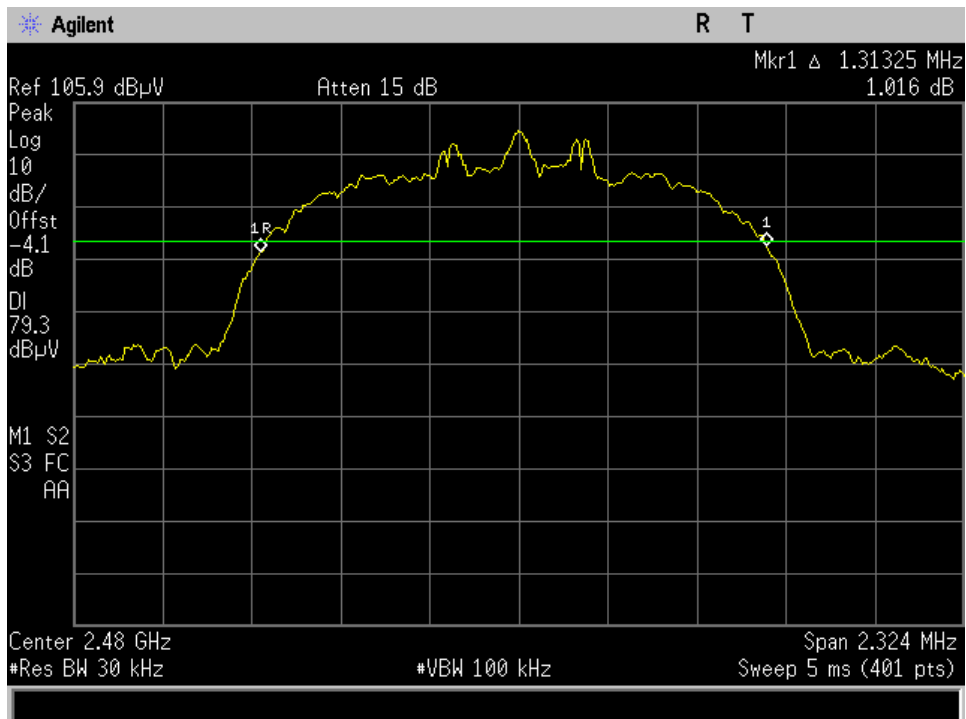
high ch DH5 20dB and 99%
