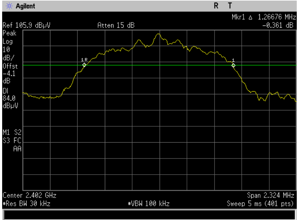
low ch DH3 20dB and 99%
