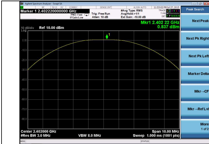
Peak Output Power – Low Channel
