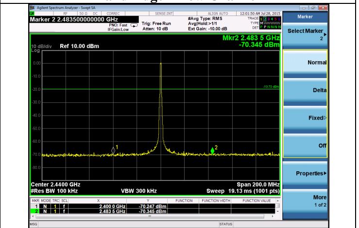
Band-Edge – Mid Channel
