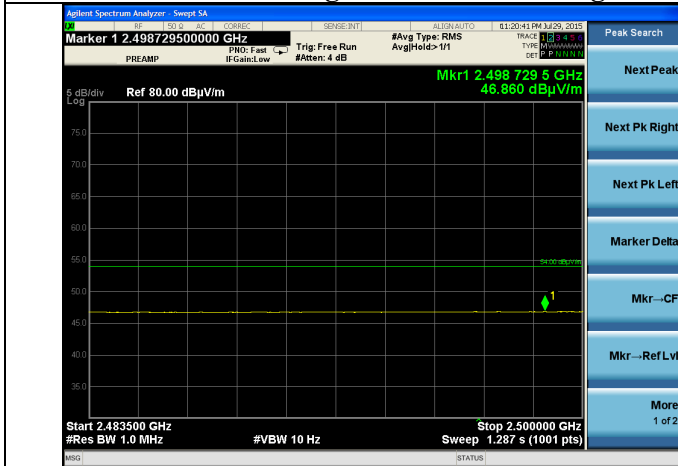
Upper Band-Edge – High Ch. - Average
