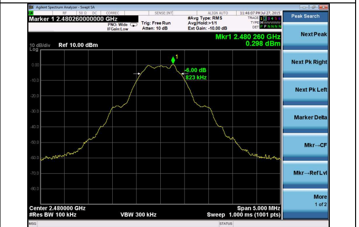
PPSD – High Channel
