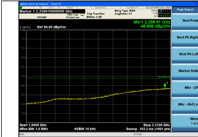
1-2.31 GHz – Average
