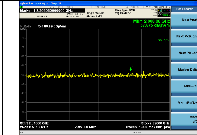
Lower Band-Edge – Low Ch. - Peak
