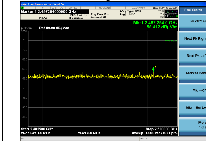
Upper Band-Edge – High Ch. - Peak
