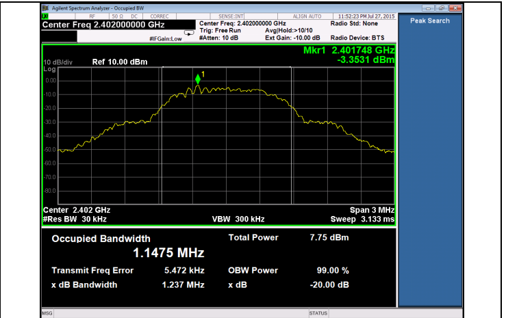
OBW + 99% BW – Low Channel
