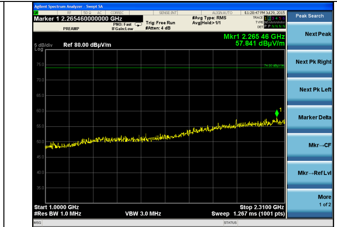
1-2.31 GHz - Peak
