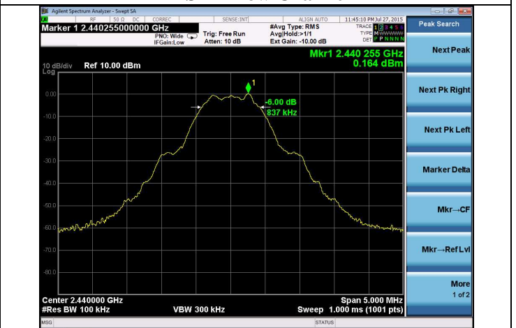
PPSD – Mid Channel
