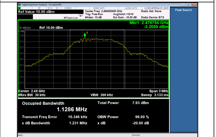
OBW + 99% BW – High Channel
