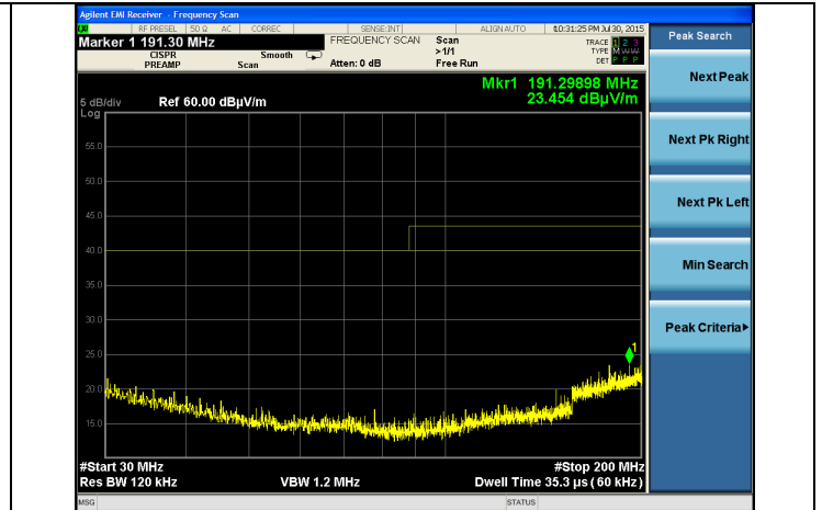
30-200 MHz - Horizontal Polarity
