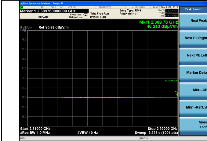
Lower Band-Edge – Low Ch. - Average
