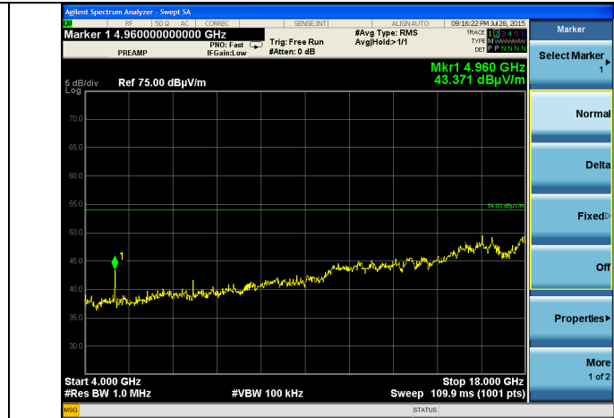
4-18 GHz – Average – Horizontal
