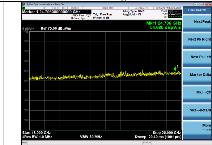
18-25 GHz - Peak
