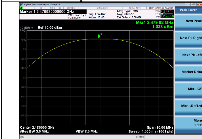
Peak Output Power – High Channel
