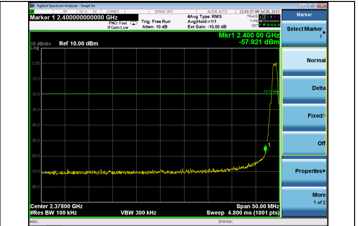
Band-Edge – Low Channel
