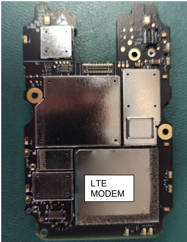
Main PCB Back
