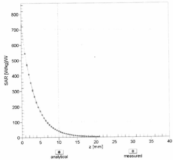
f = 5750 MHz, WGLS R58 (H_convF)-SCS
