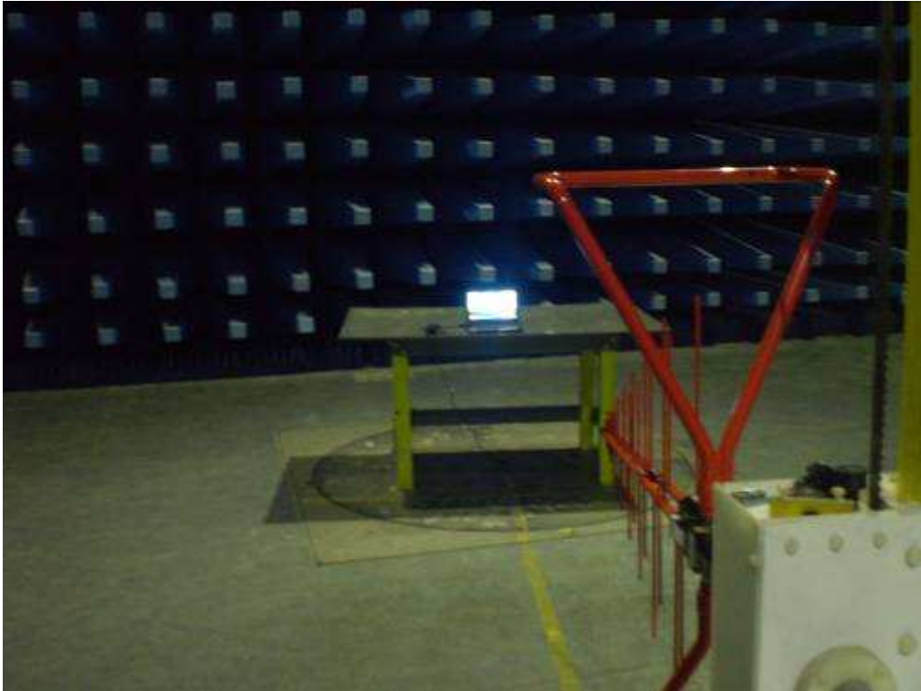
Radiated Emission Front View below 1GHz
